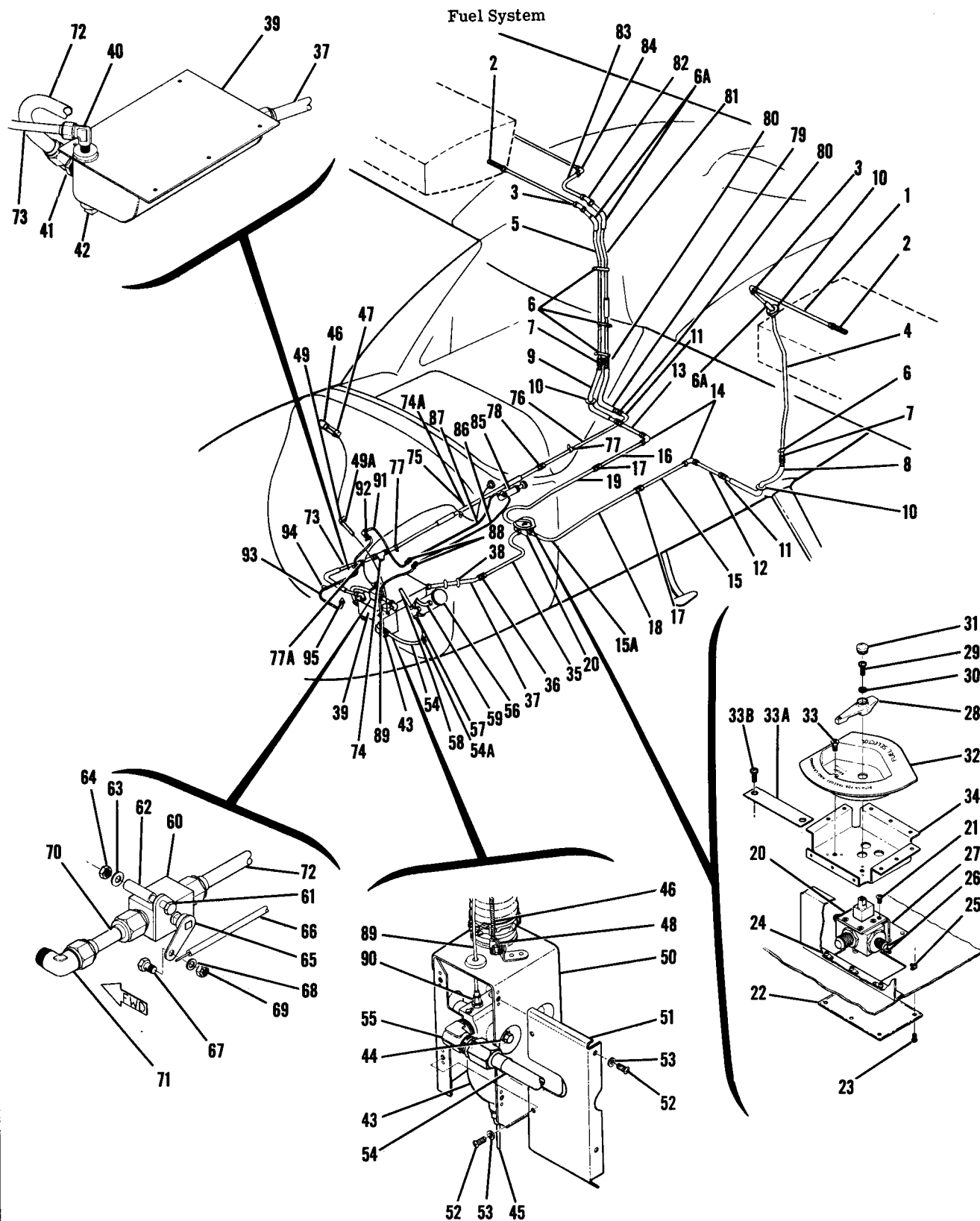
Figure 69. Fuel System Installation
