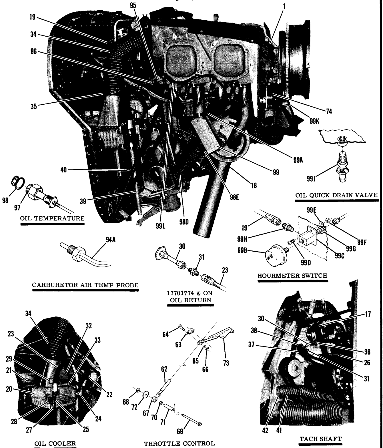
Figure 51A. Engine Installation (Sheet 2 of 2)
