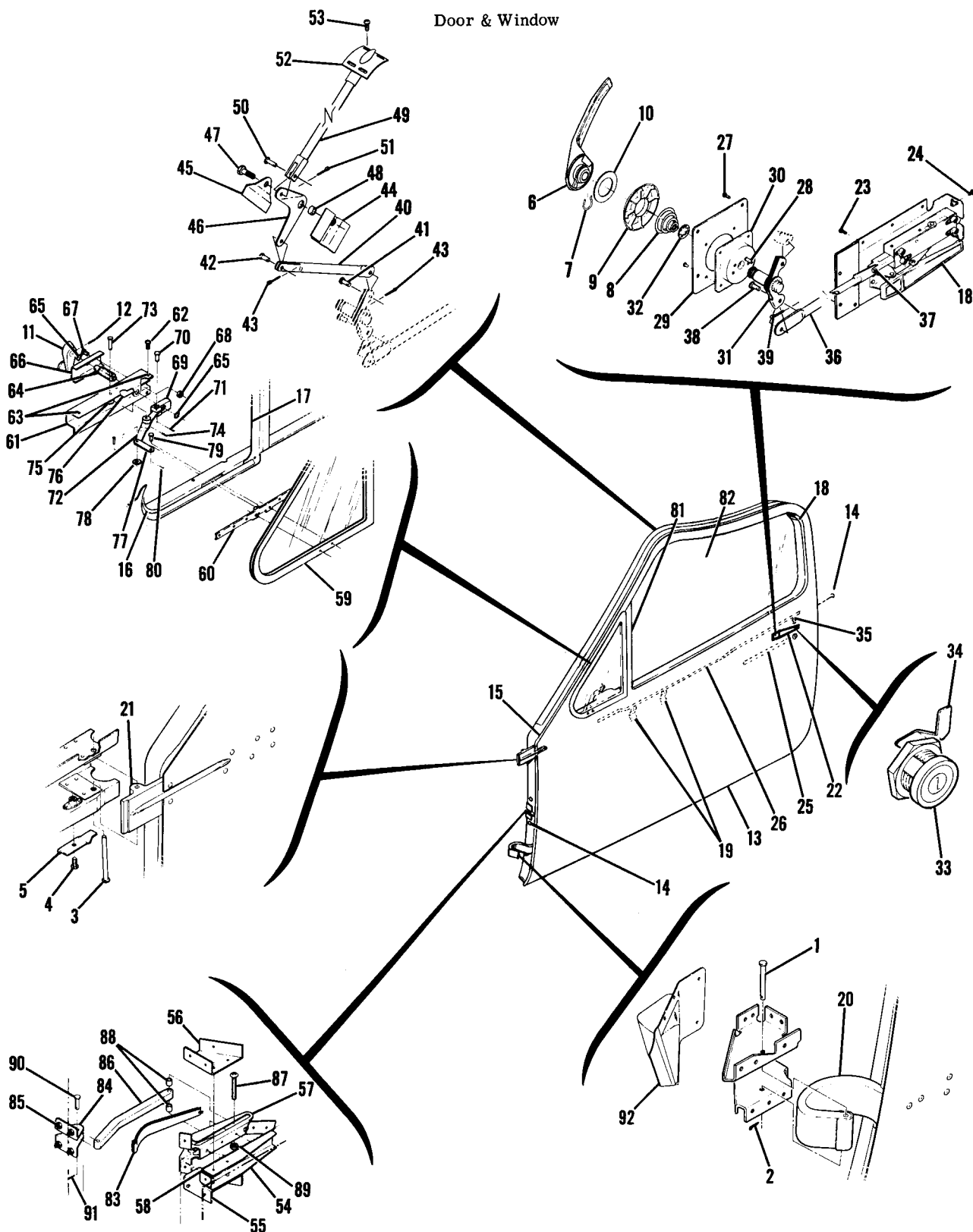
Figure 35A. Cabin Door Assembly
