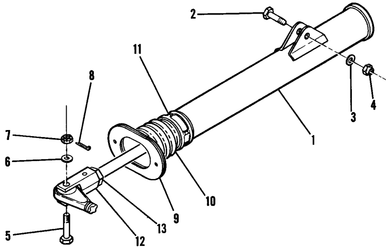
Figure 27. Nose Gear Steering Rod Installation
