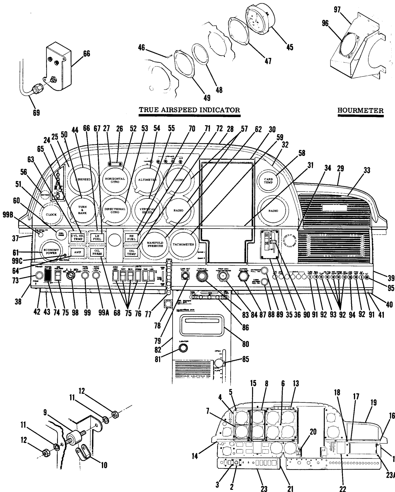
Figure 45D. Instrument Panel Equipment Installation
