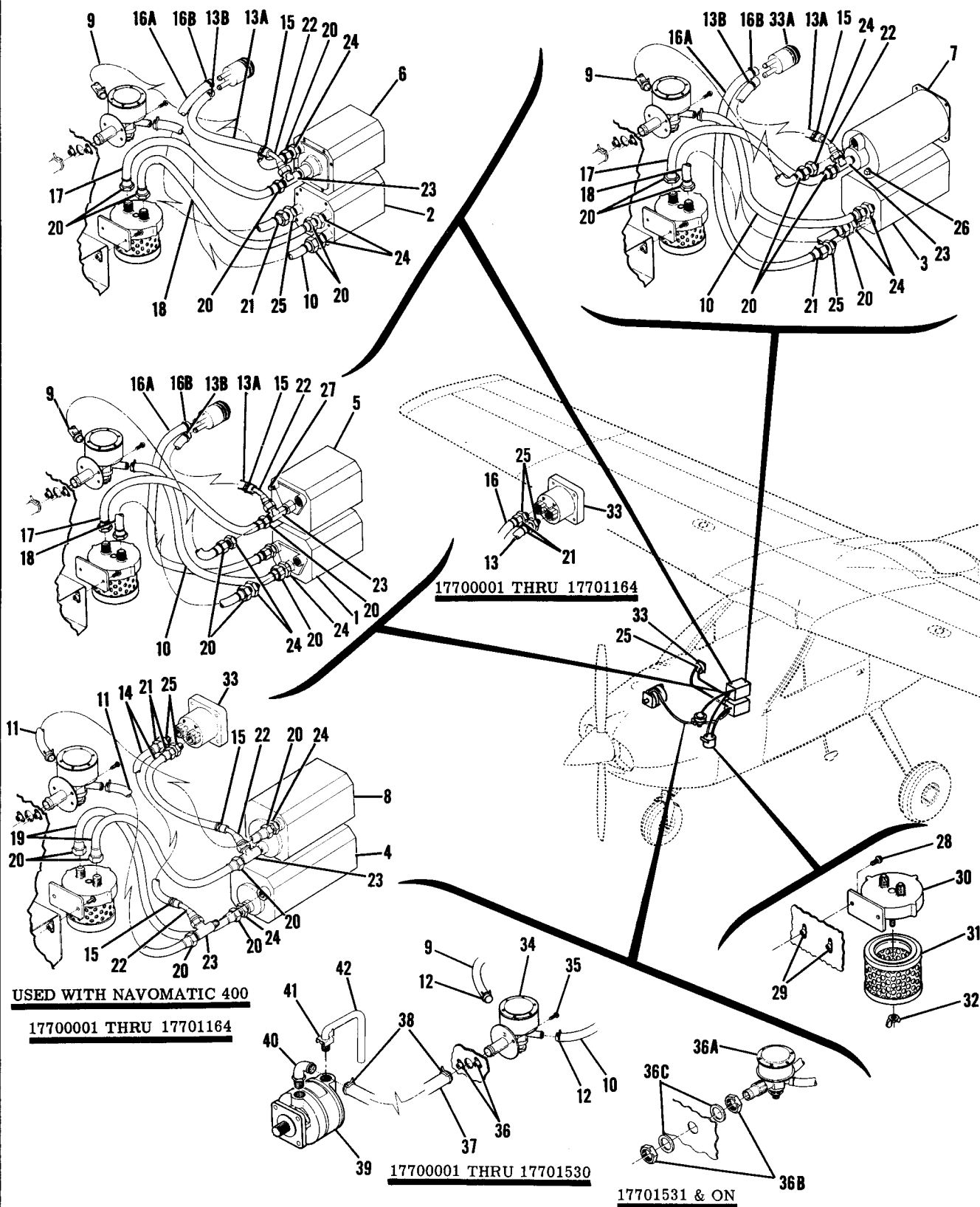
Figure 74. Vacuum System Installation
