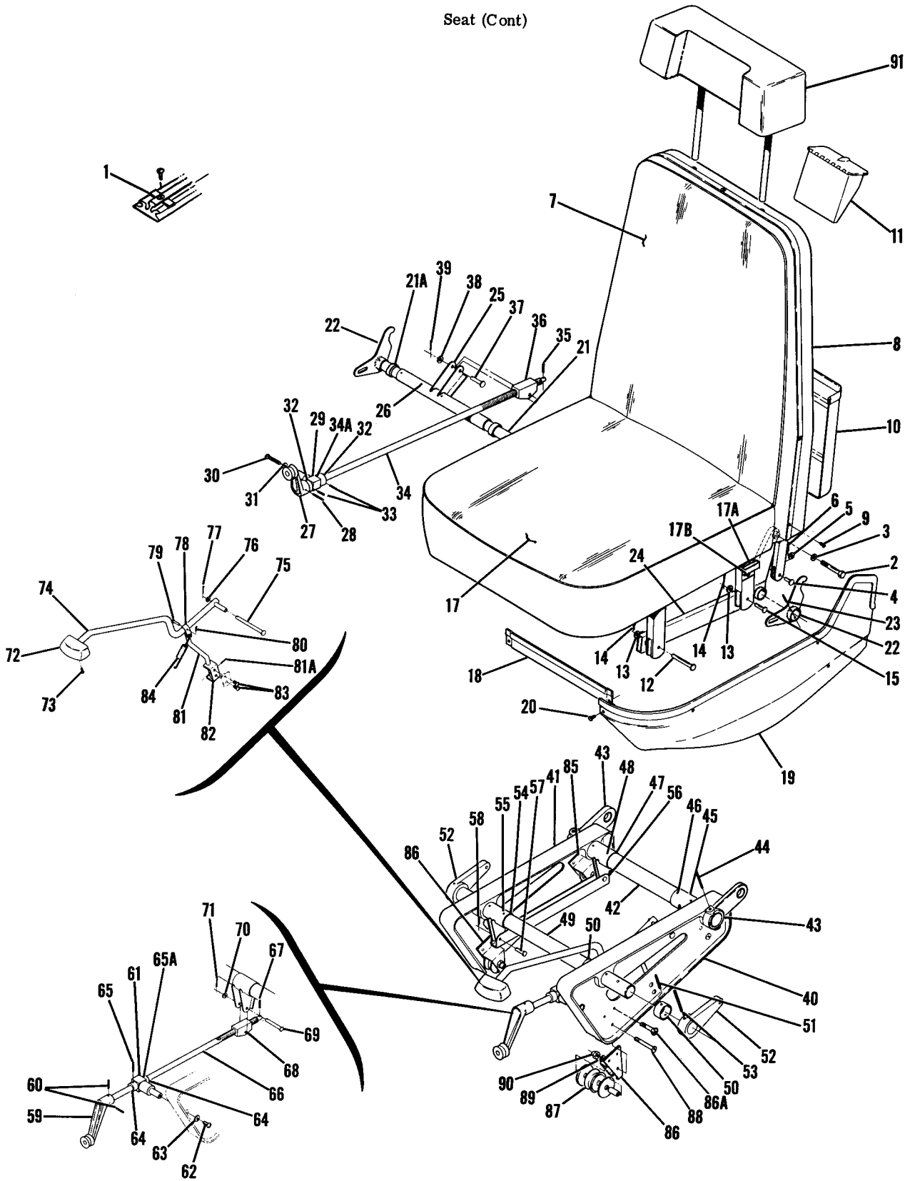
177 SERIAL 17701371 THRU 17701773 Figure 42A. Infinitely Adjustable Front Seat Installation
