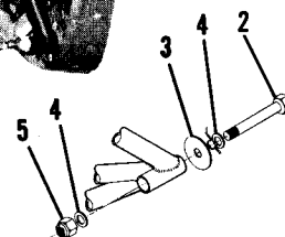
ENGINE MOUNT
