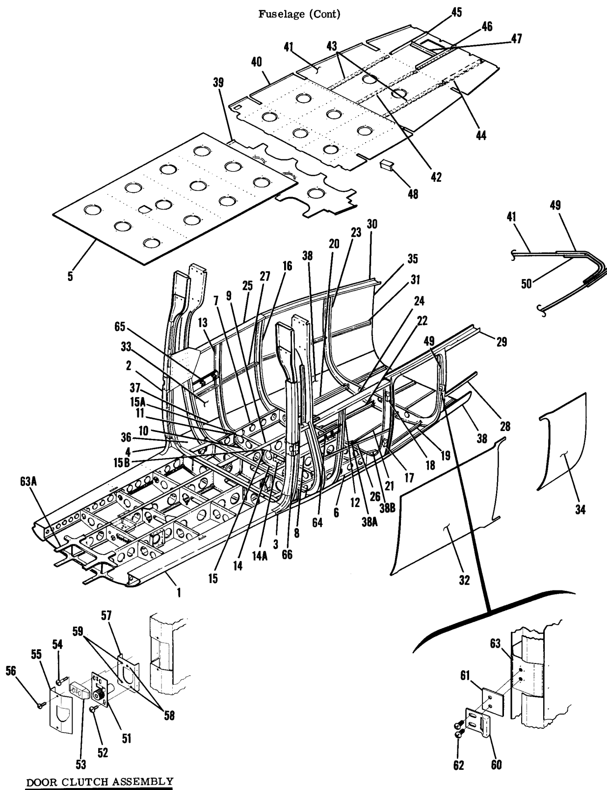
Figure 17. Center Cabin Section-Lower
