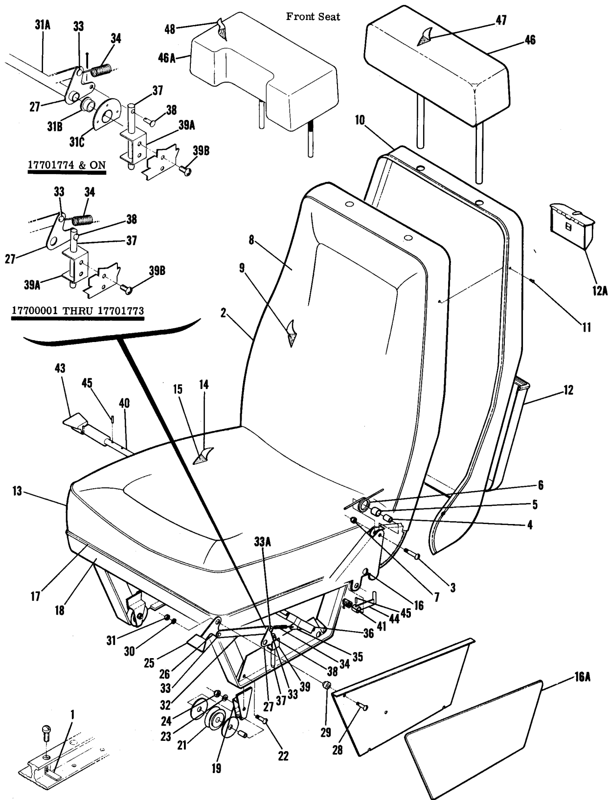
Figure 41. Front Seats Installation
