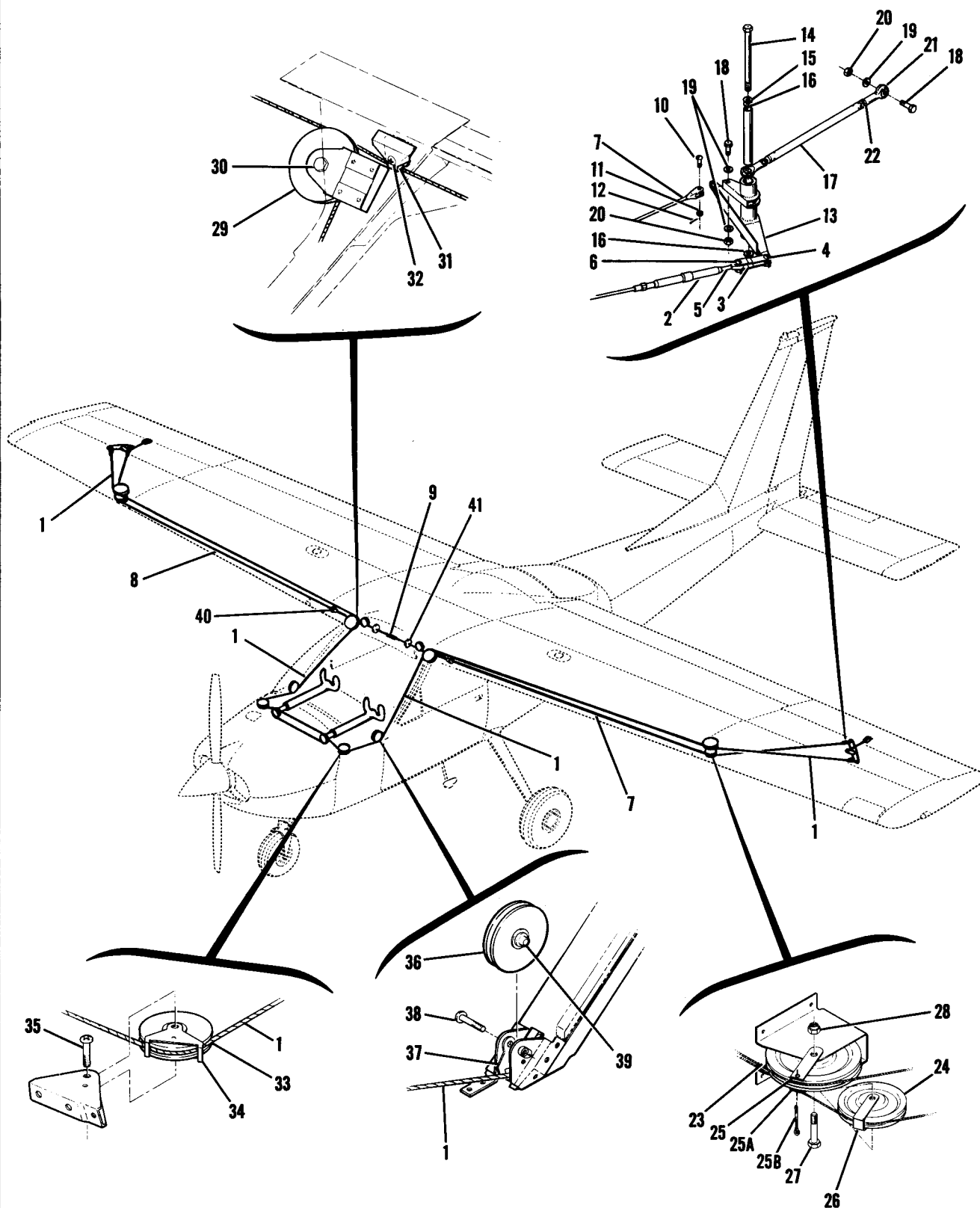
Figure 62. Aileron Control System
