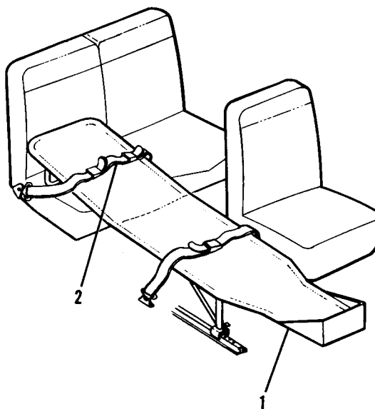
Figure 47. Stretcher Installation
