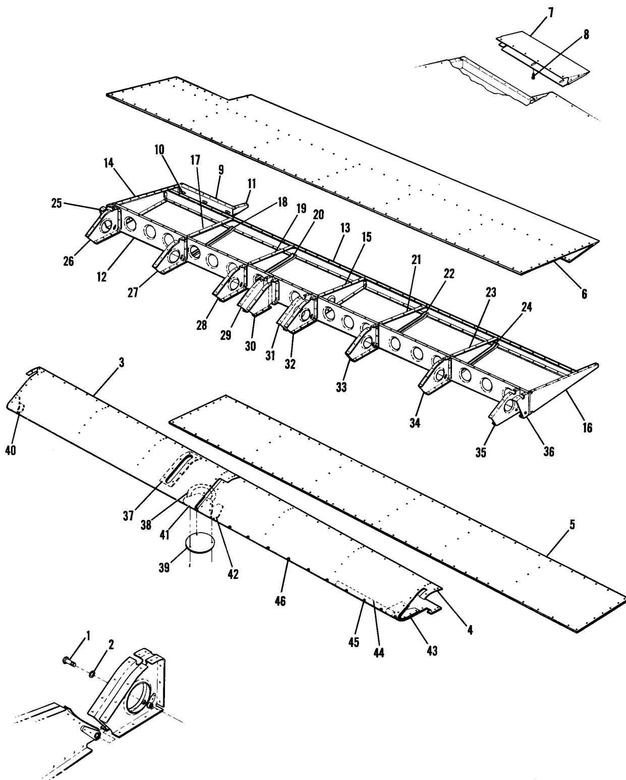
Figure 7. Aileron Installation
