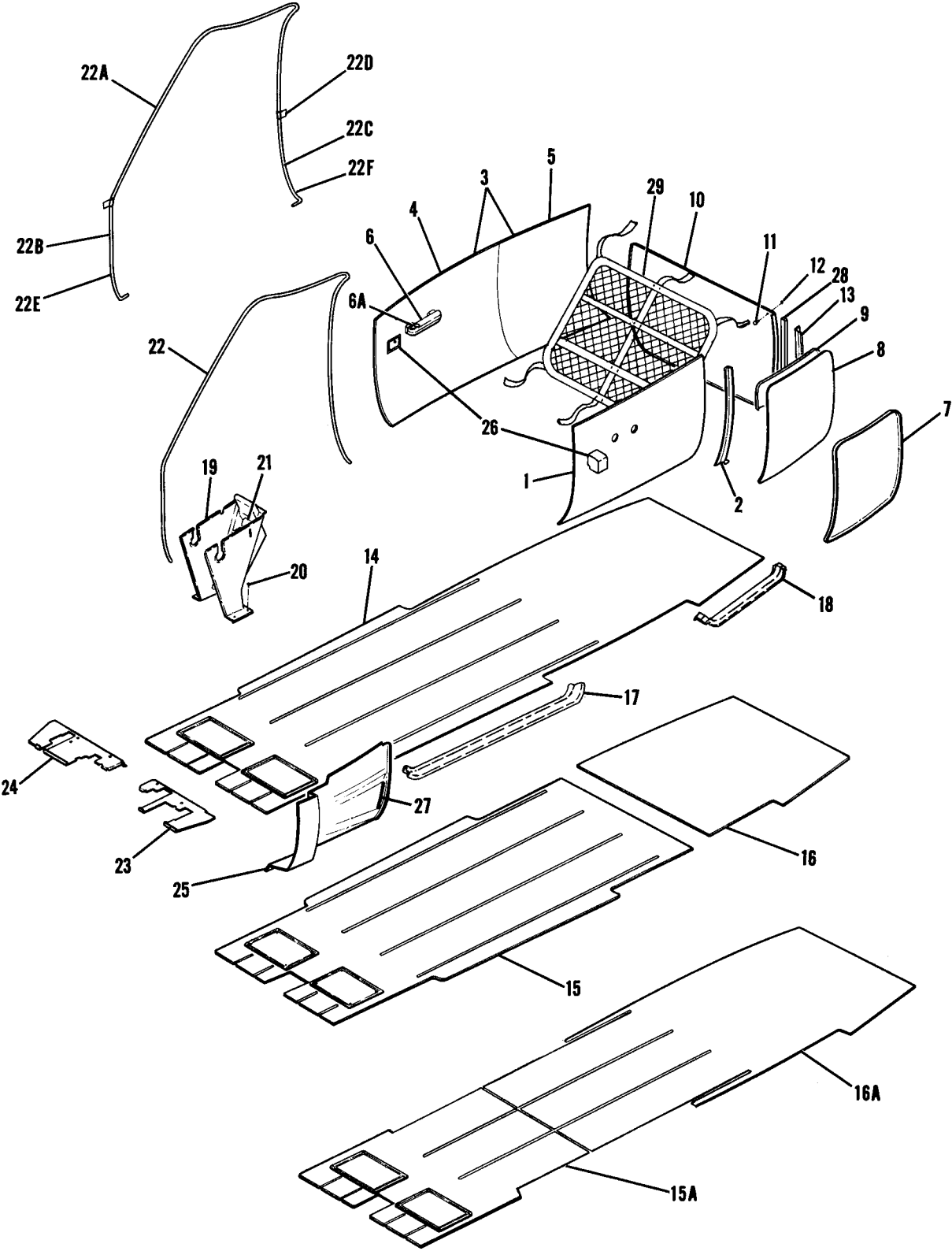
Figure 40. Cabin Side & Floorboard Upholstery Installation
