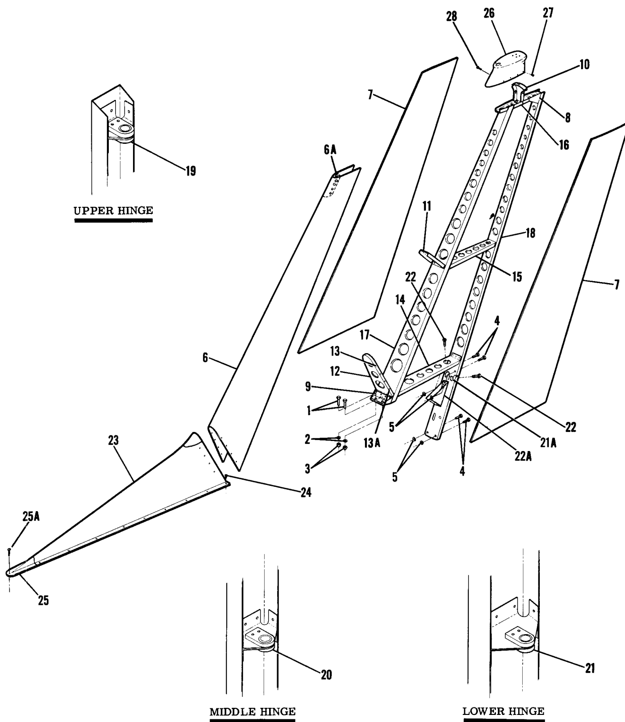
Figure 9. Vertical Fin & Dorsal Installation
