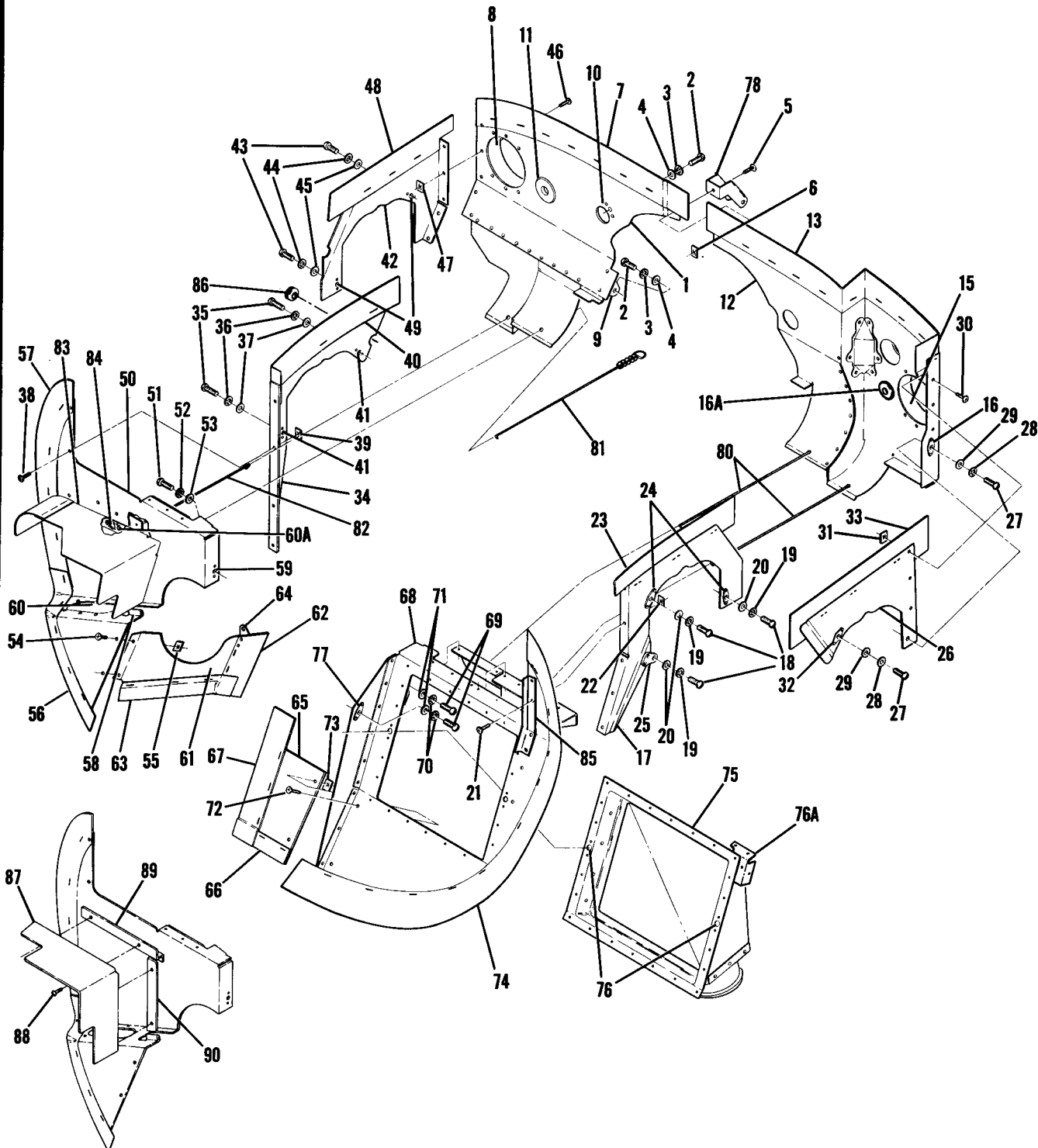
Figure 54A. Engine Baffles Installation
