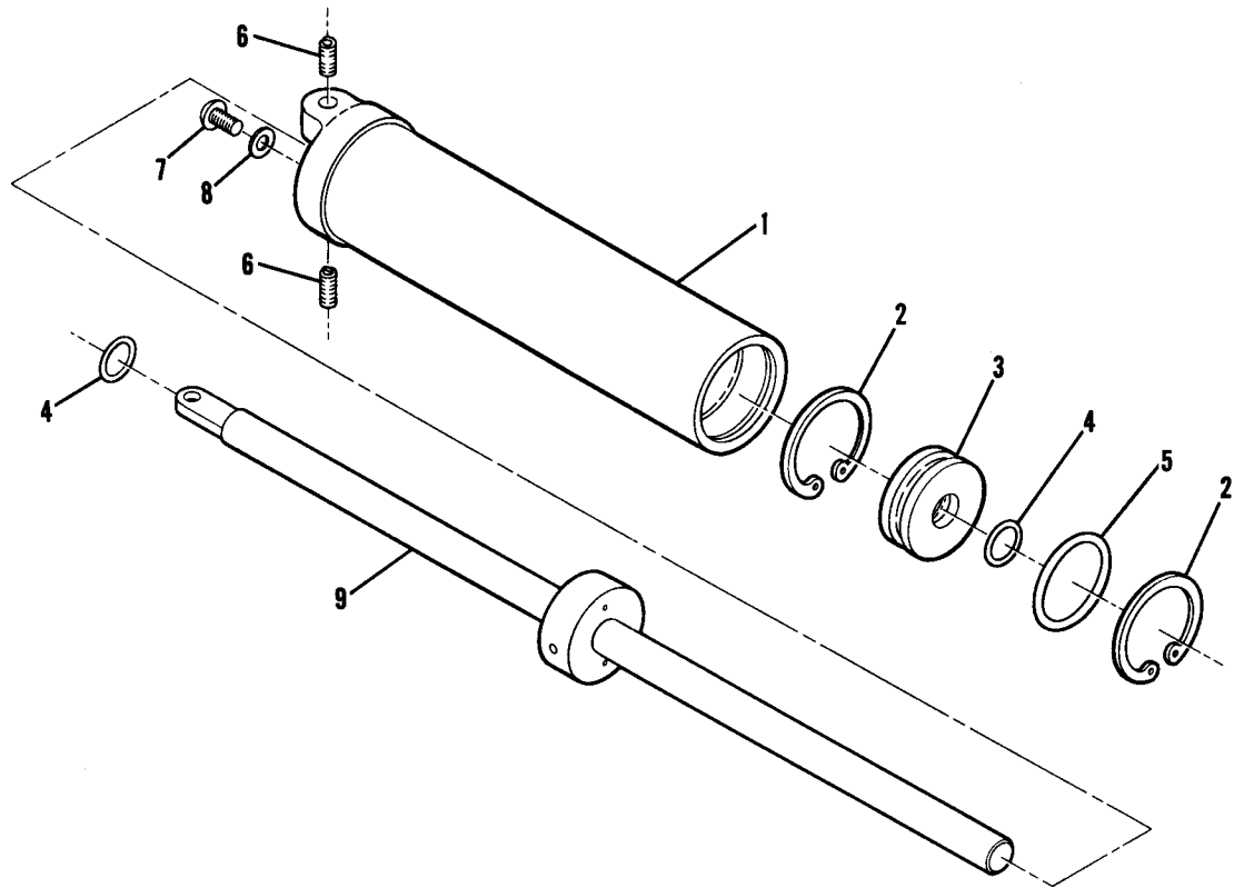
Figure 32. Shimmy Dampener Assembly
