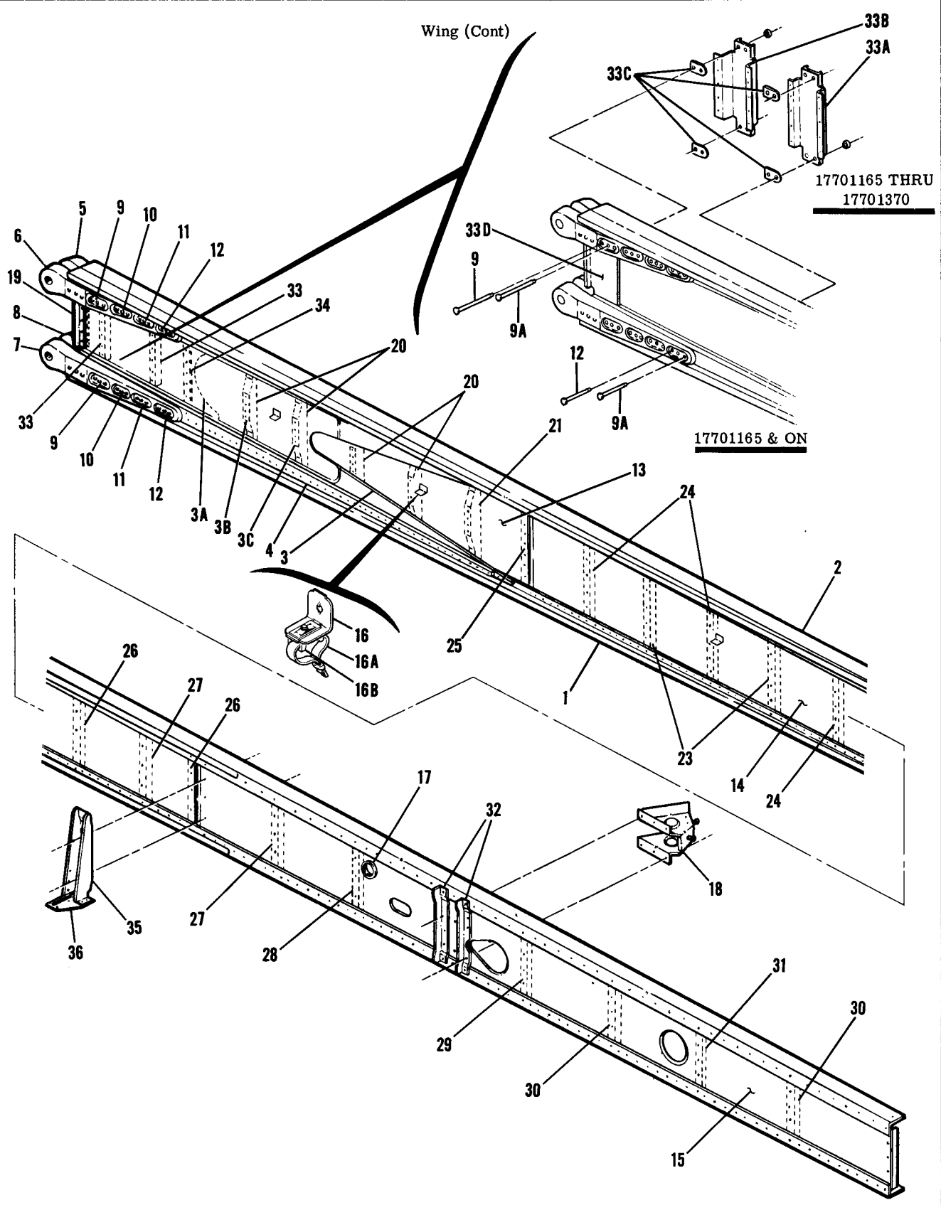
Figure 6. Wing Main Spar Assembly
