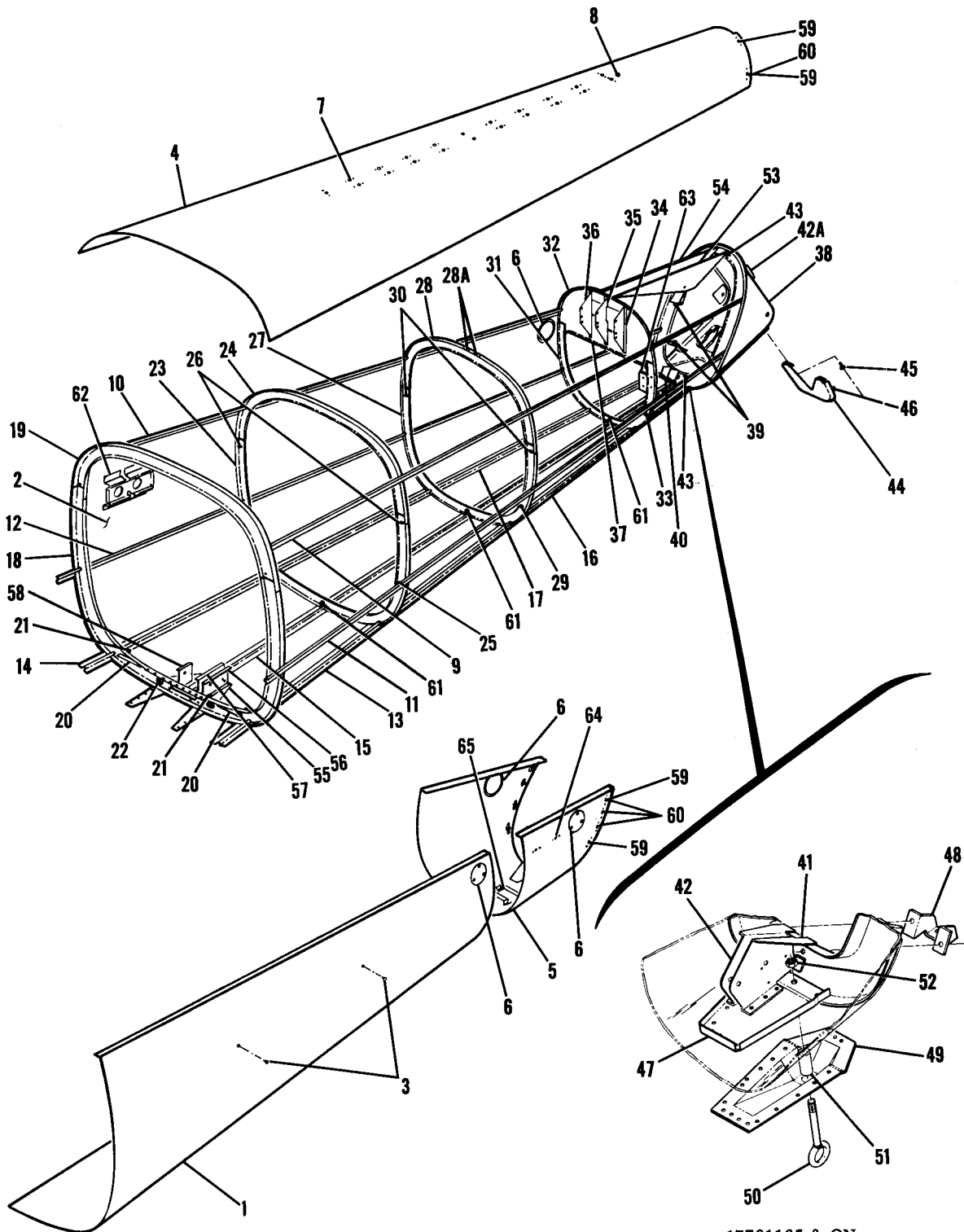
Figure 22. Tailcone Assembly
