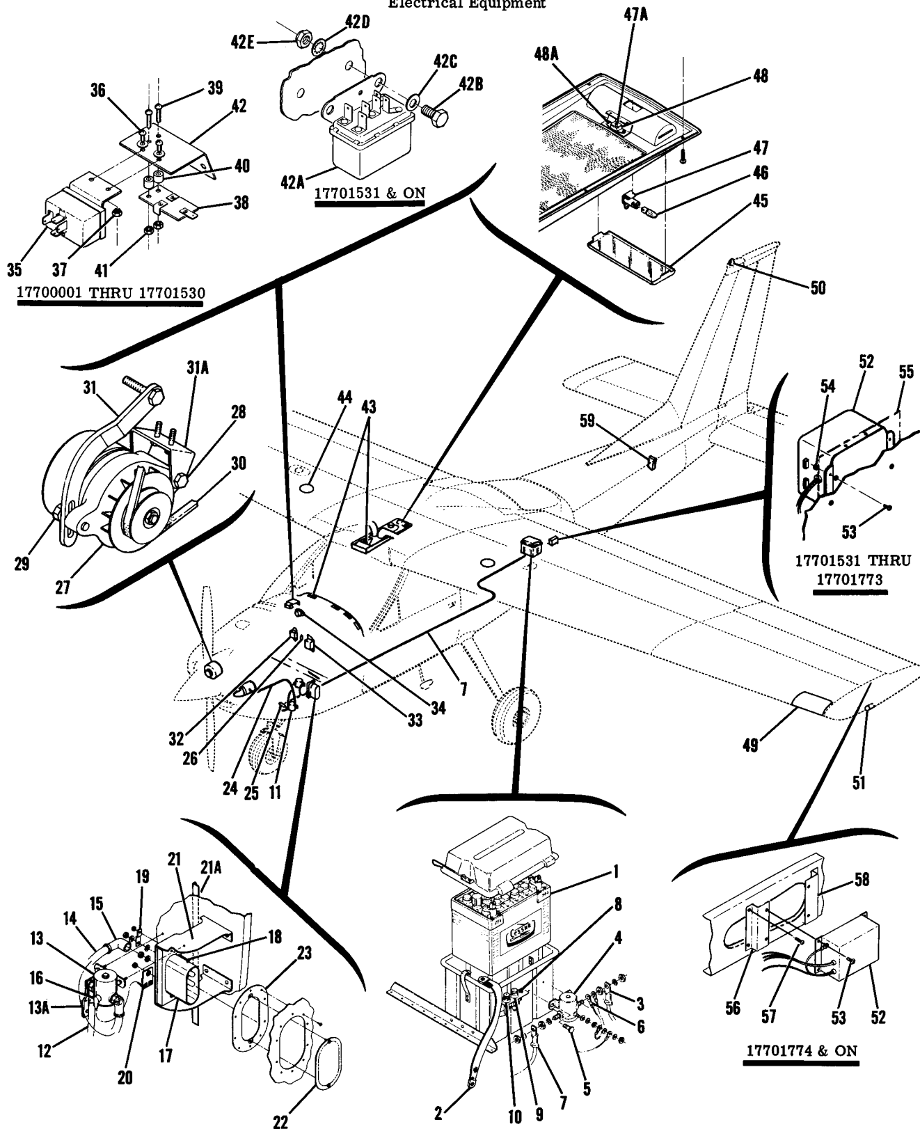
Figure 76. Electrical Equipment Installation
