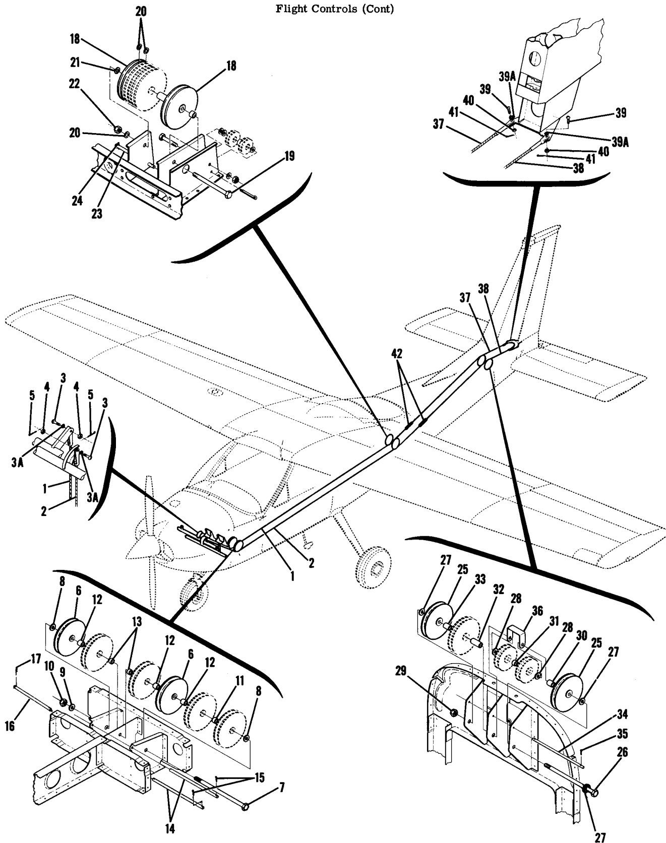
Figure 66. Rudder Control System Installation
