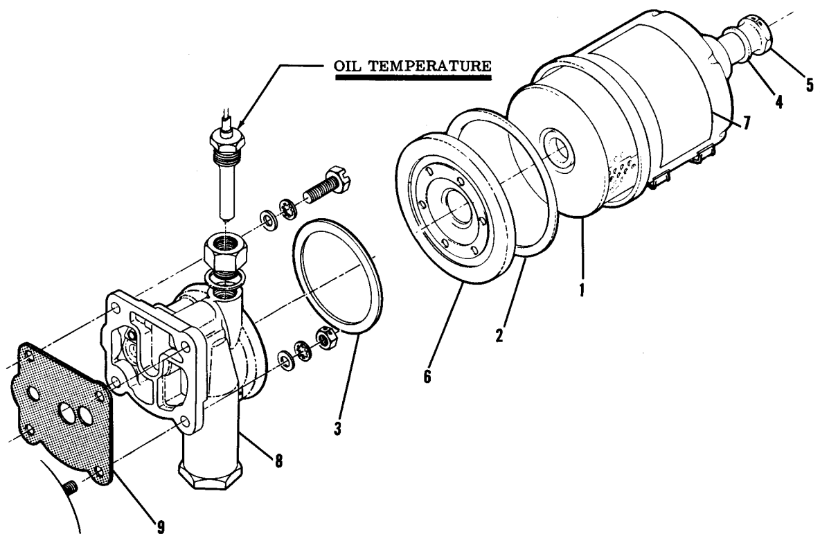
Figure 55. Oil Filter Installation
