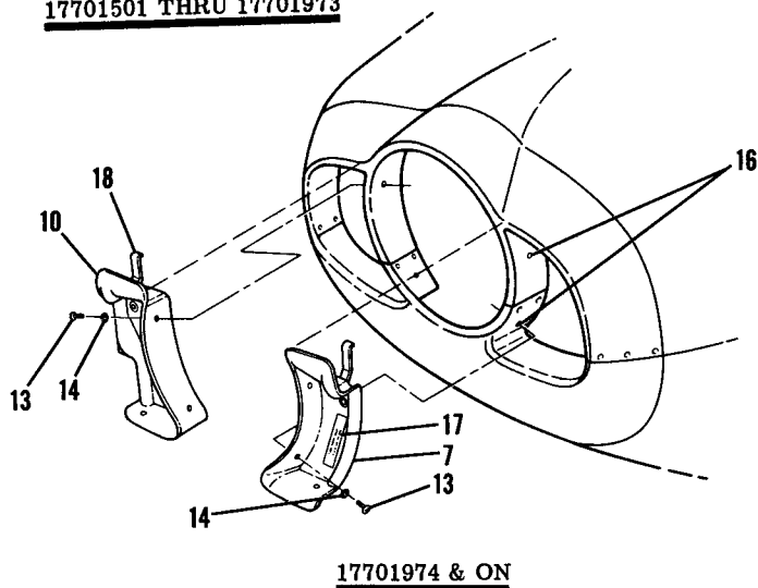
Figure 50. Winterization Equipment Installation
