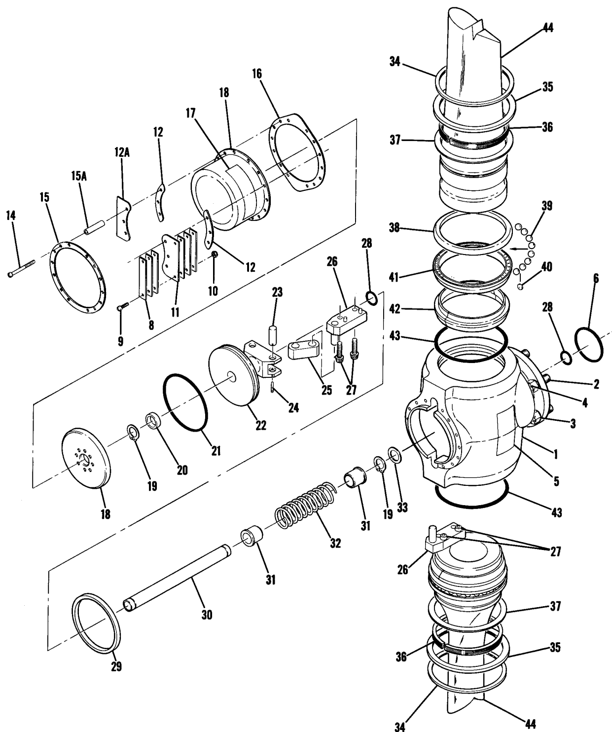
Figure 48B. McCauley Propeller Assembly
