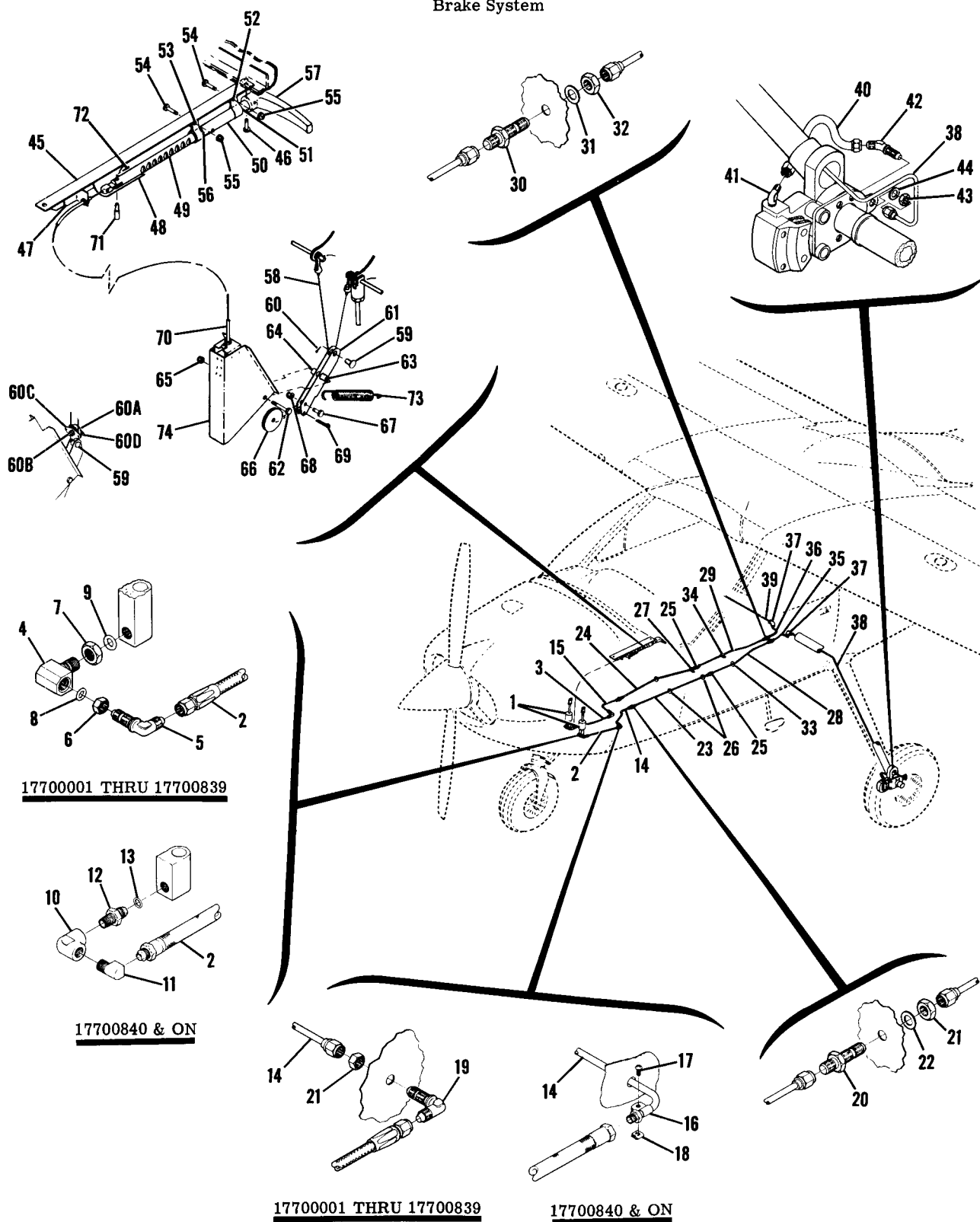
Figure 58. Brake System Installation
