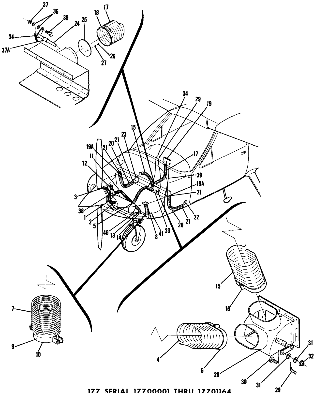
Figure 57. Heating &amp; Defrosting System
