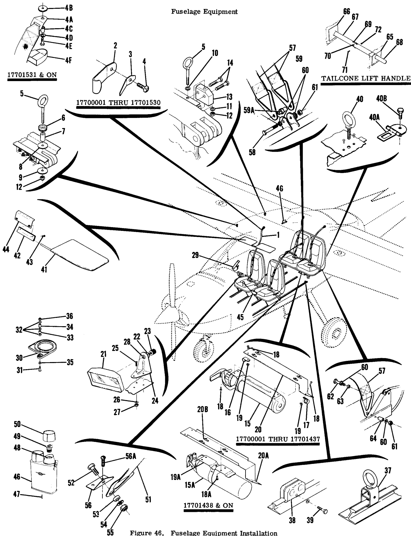
Figure 46. Fuselage Equipment Installation
