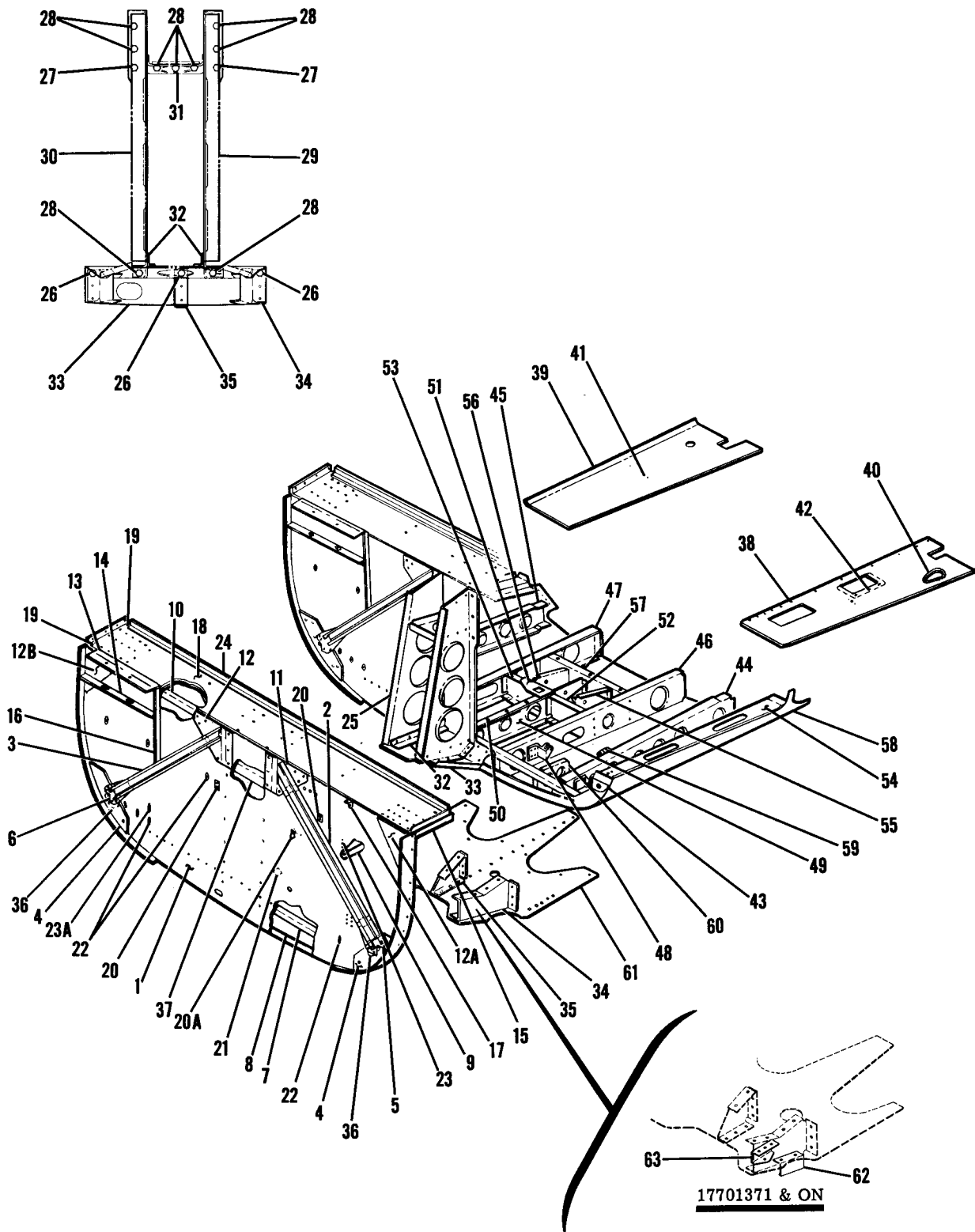
Figure 16. Lower Forward Fuselage Section
