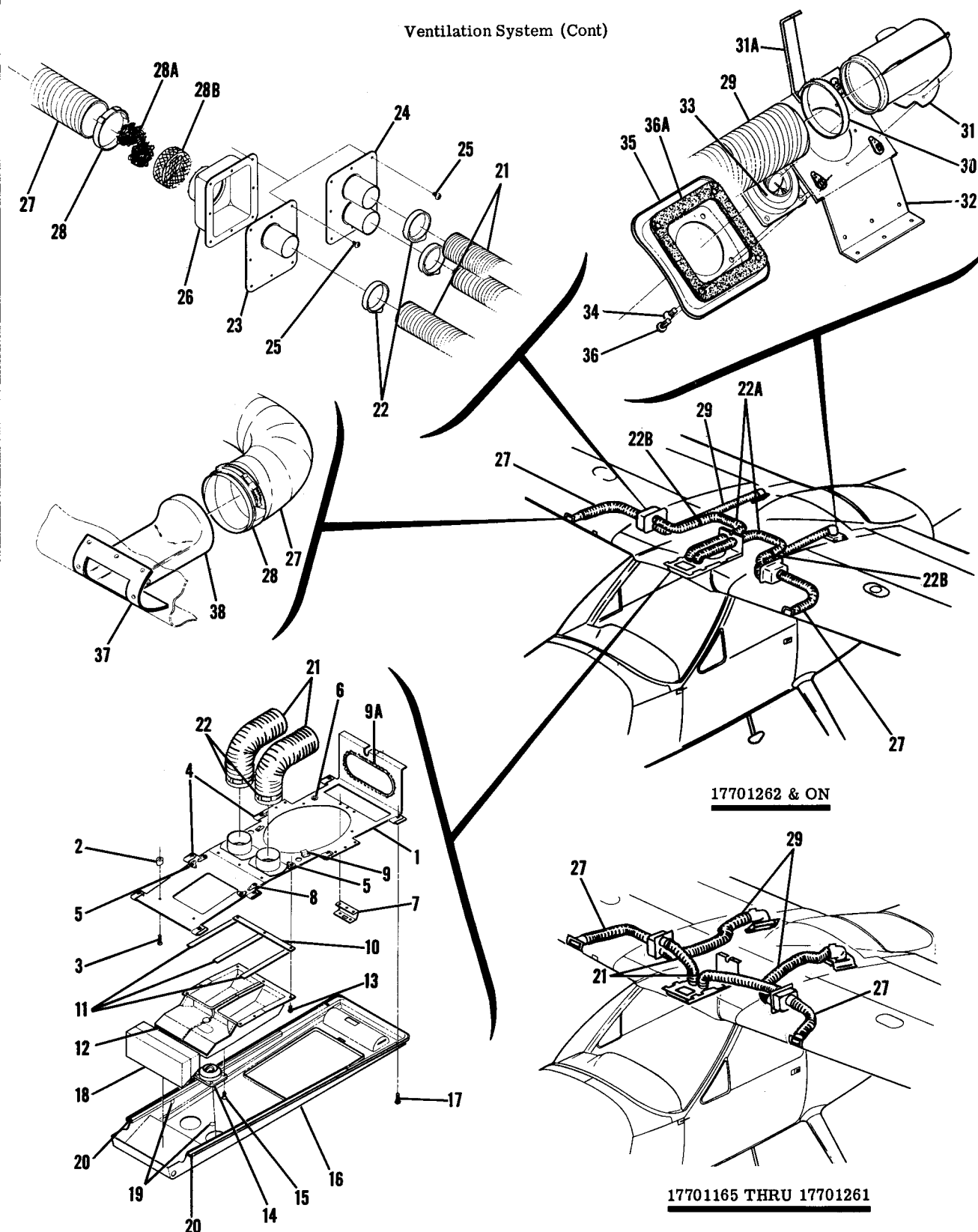
Figure 56A. Cabin Air Ventilation System Installation
