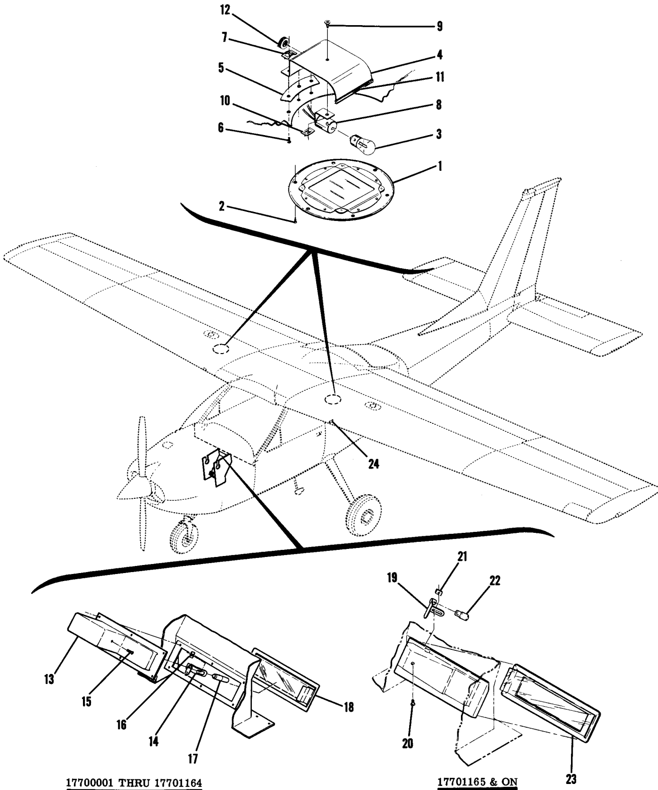
Figure 79. Courtesy Lights Installation
