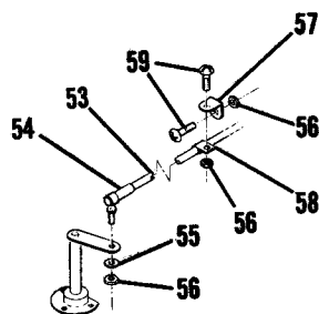
CARBURETOR HEAT CONTROL
