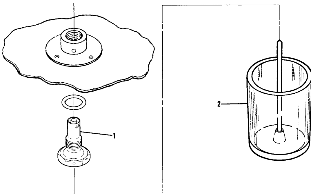
Figure 5C. Fuel Tank Drain Valve Installation
