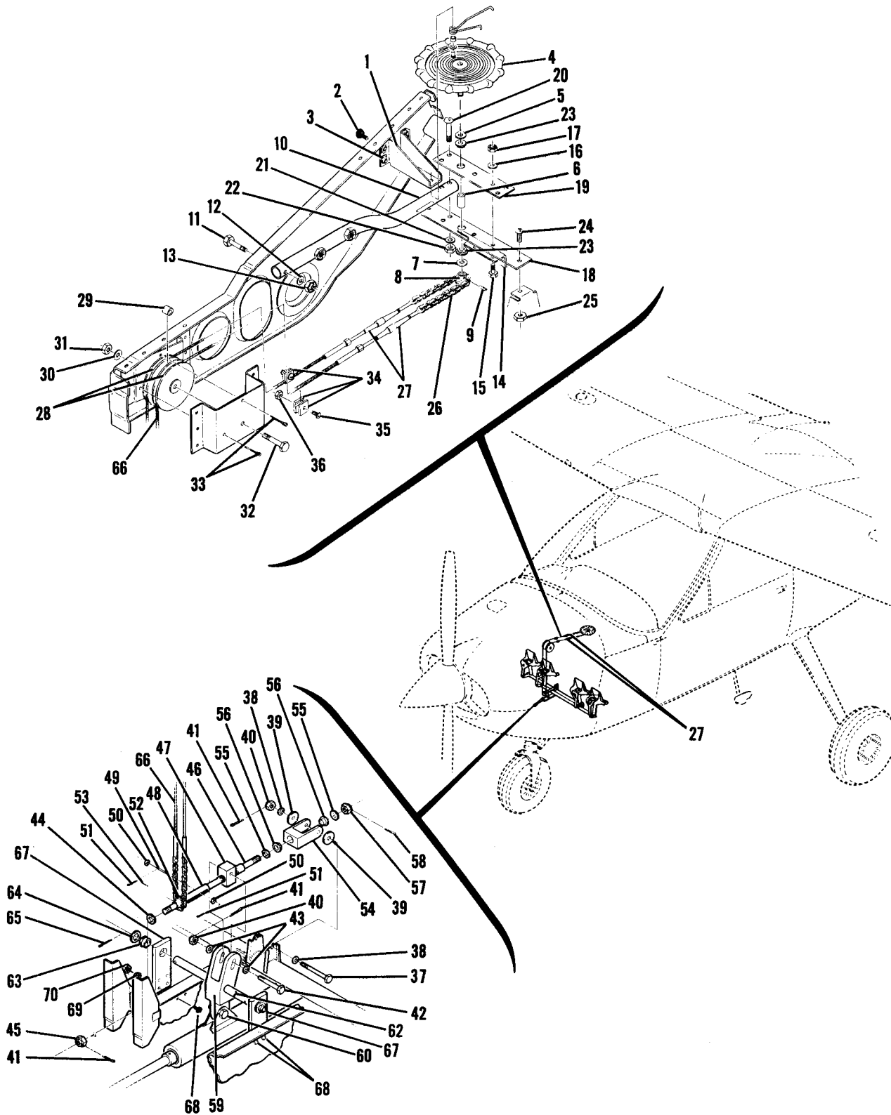
Figure 66A. Rudder Trim System Installation
