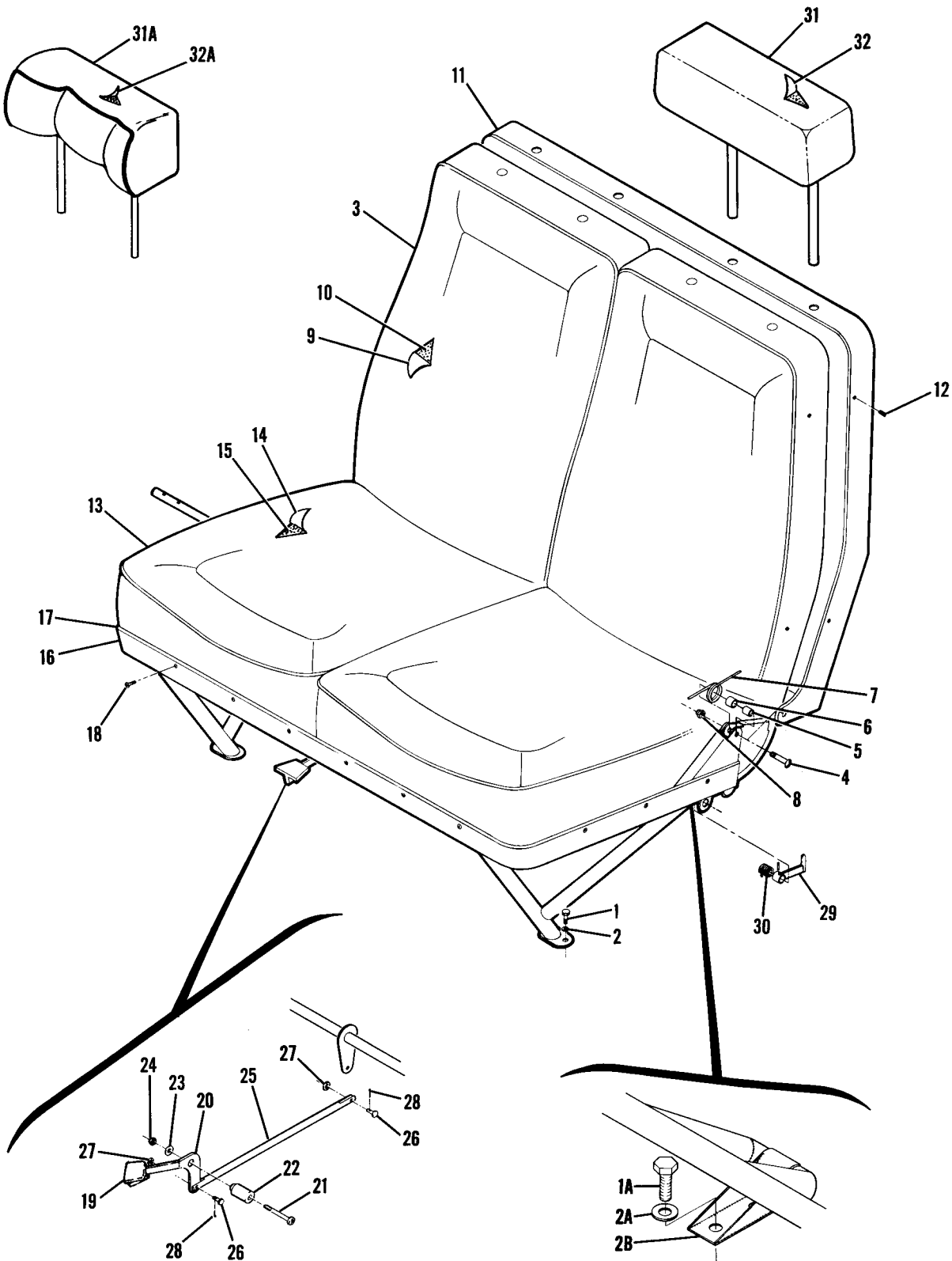
Figure 43. Rear Seat Installation
