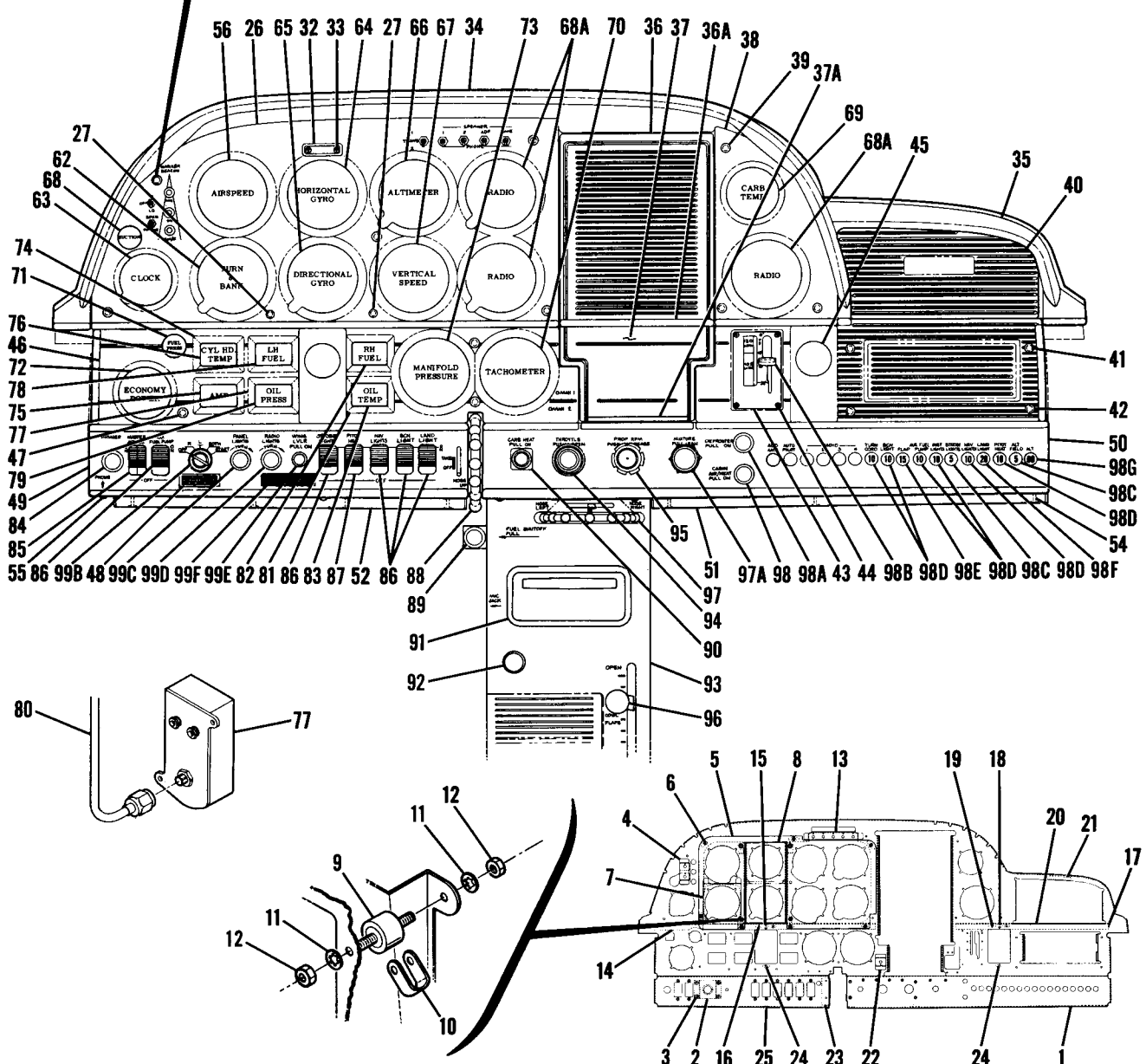
Figure 45C. Instrument Panel Equipment Installation
