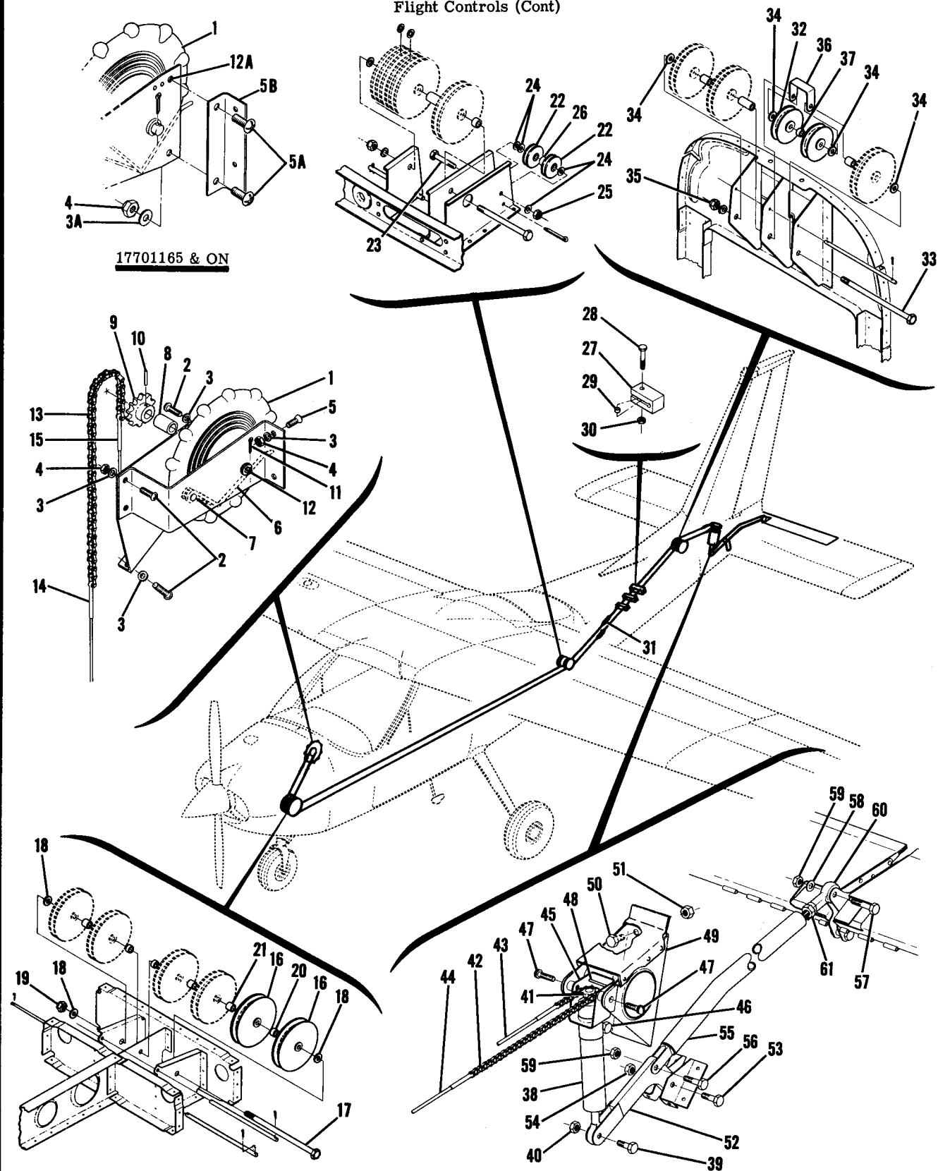
Figure 64. Stabilator Trim Tab Control System
