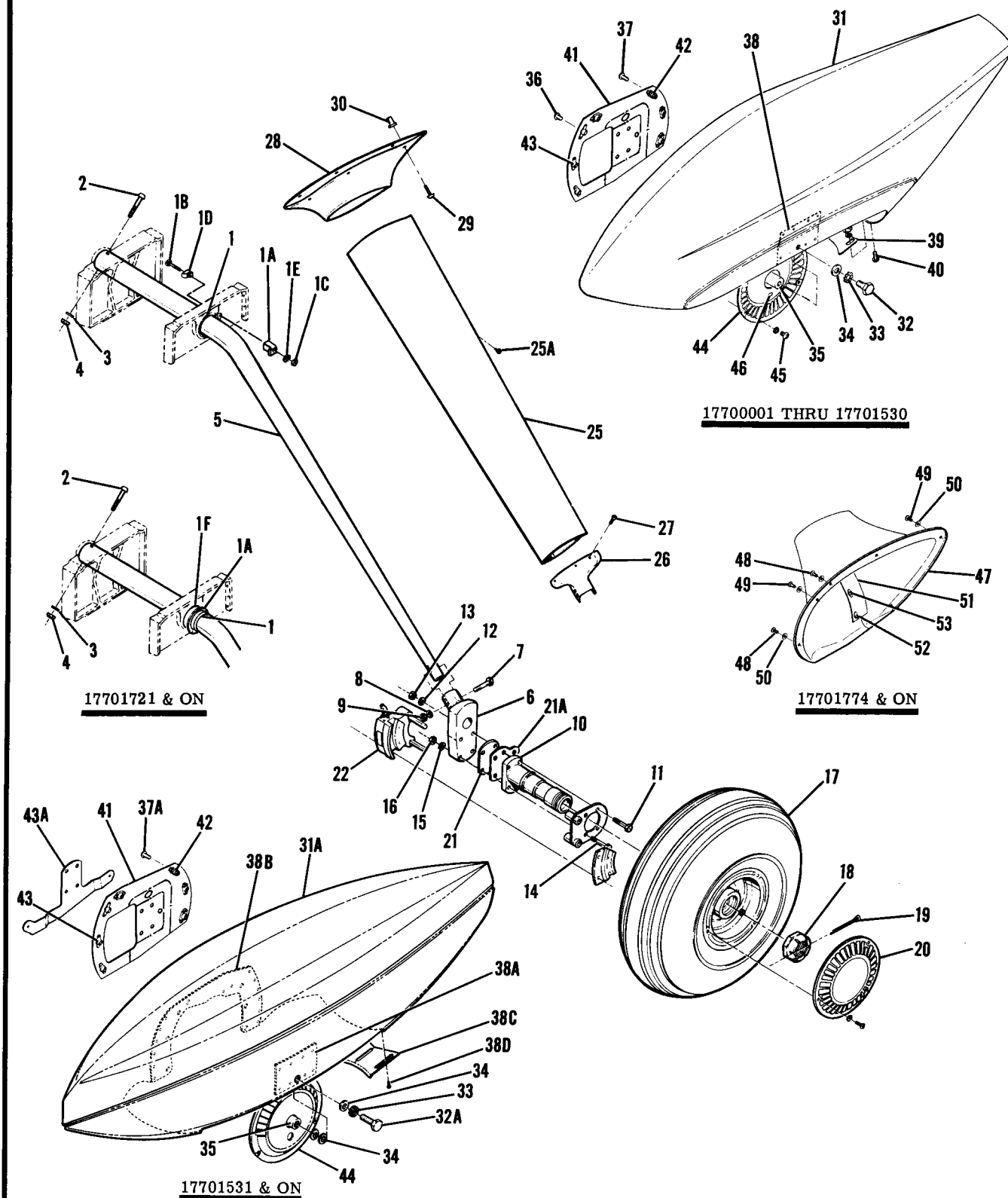
Figure 33. Main Landing Gear Installation
