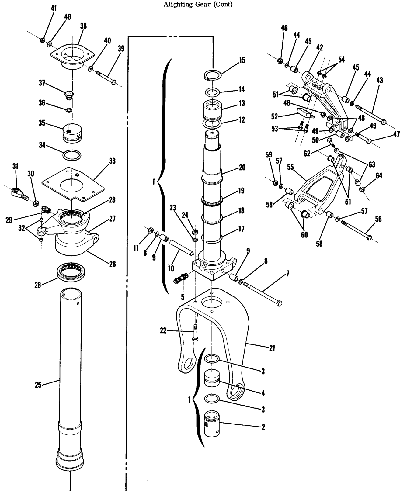
Figure 29. Nose Gear Shock Strut Assembly-Heavy Duty
