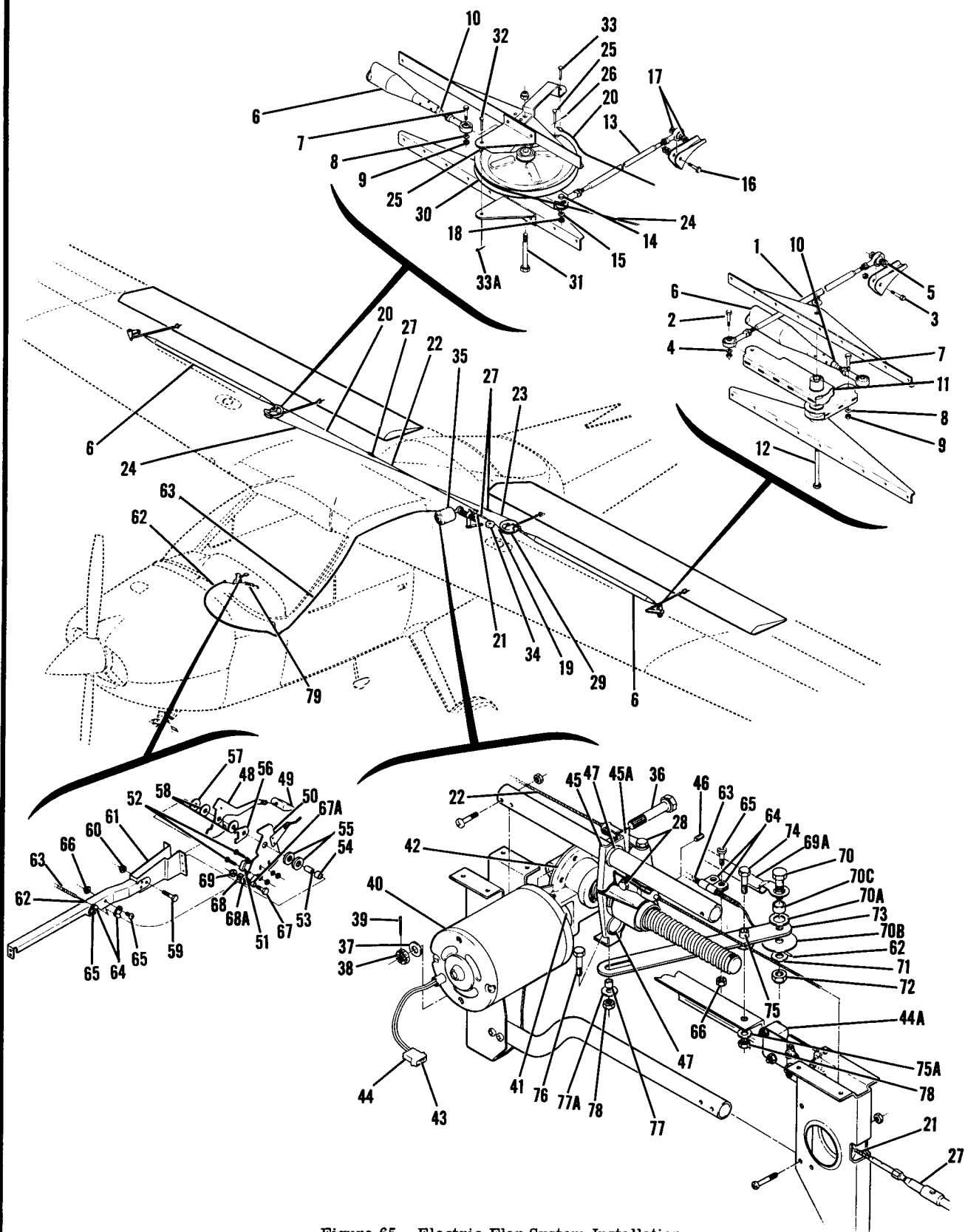
Figure 65. Electric Flap System Installation
