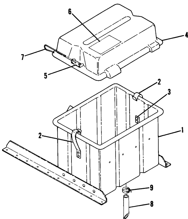
Figure 24. Battery Box Installation
