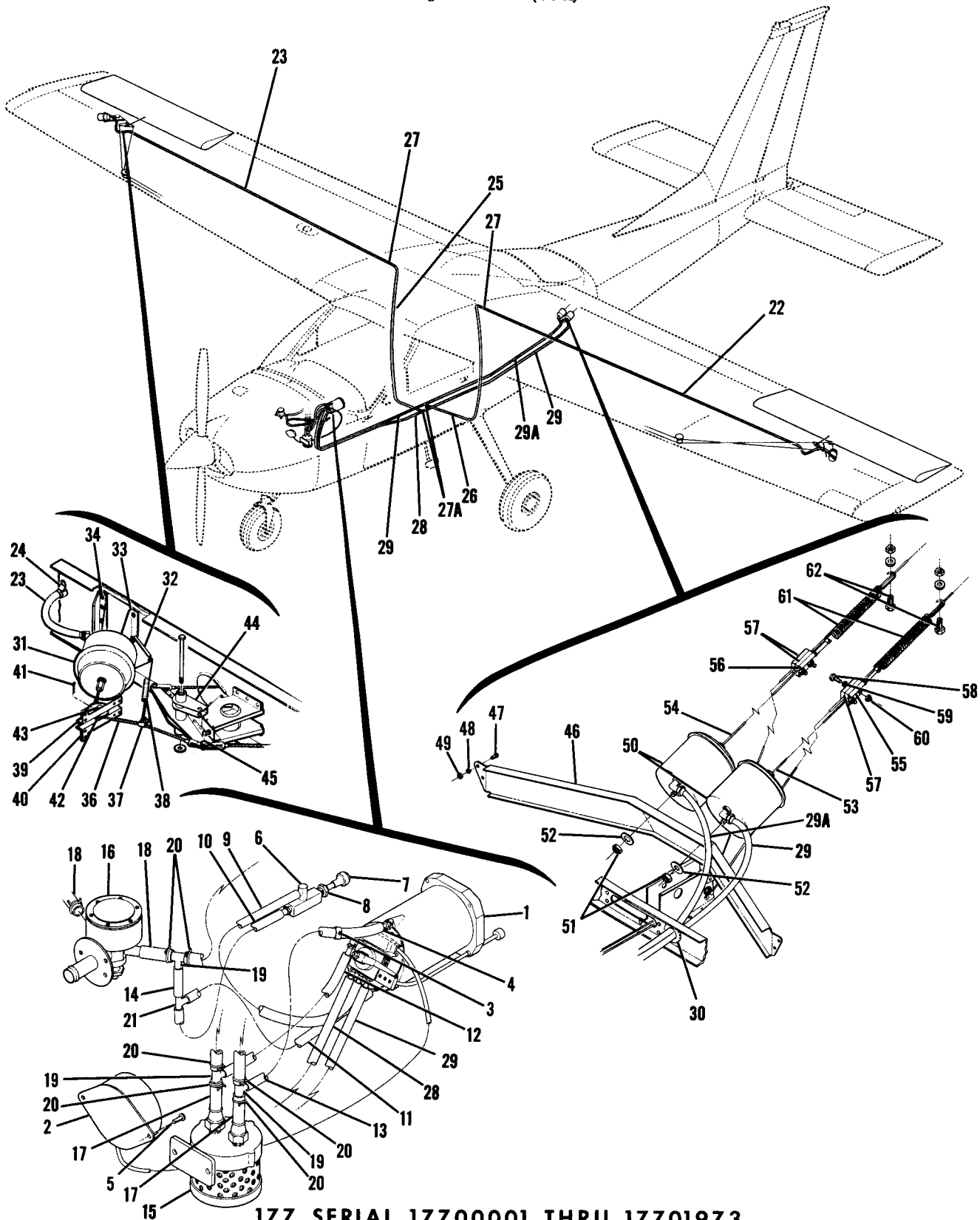
Figure 75. Wing Leveler Installation
