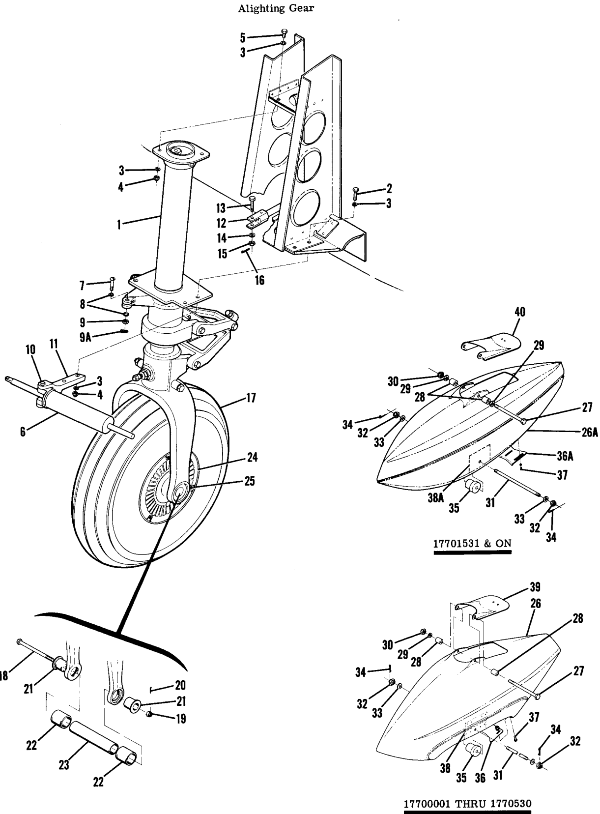
Figure 25. Nose Gear Installation
