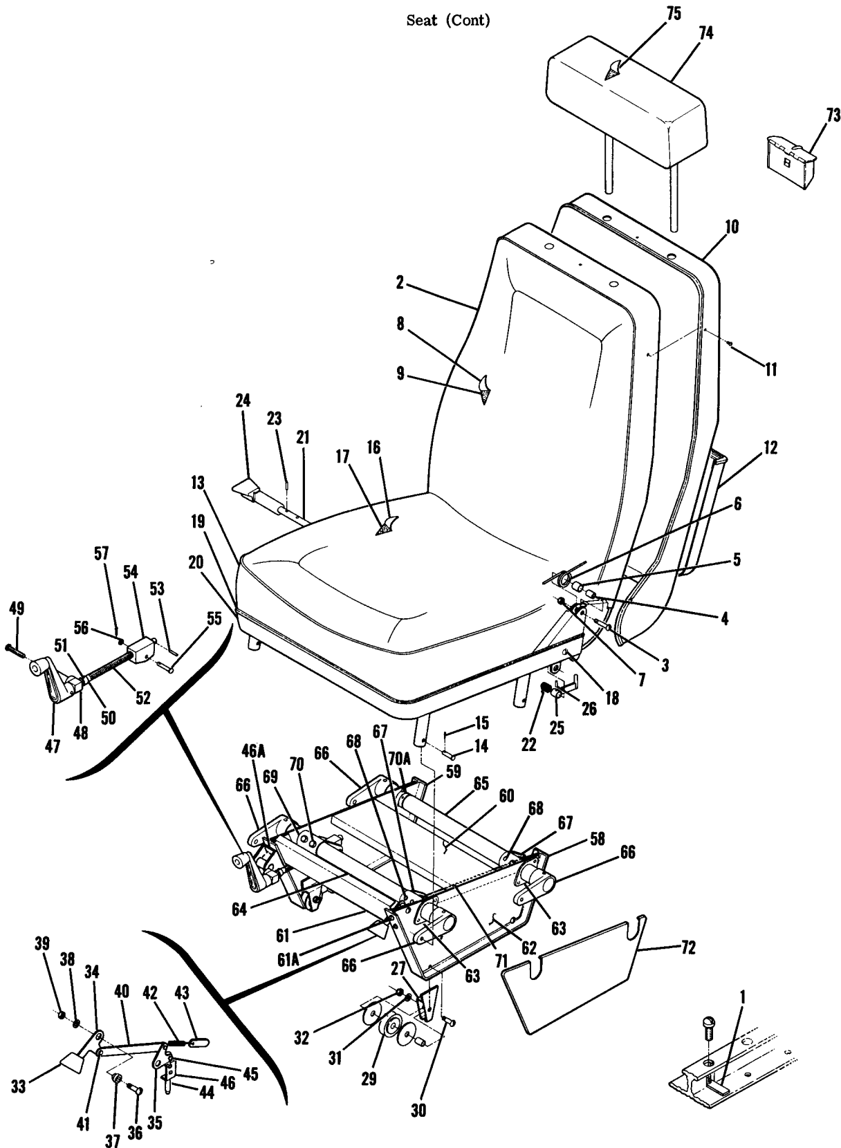
Figure 42. Vertically Adjustable Seats Installation
