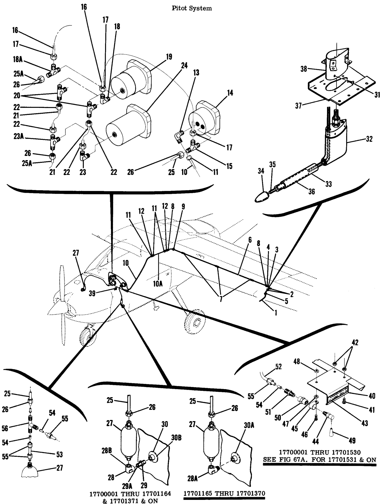
Figure 67. Pitot System Installation
