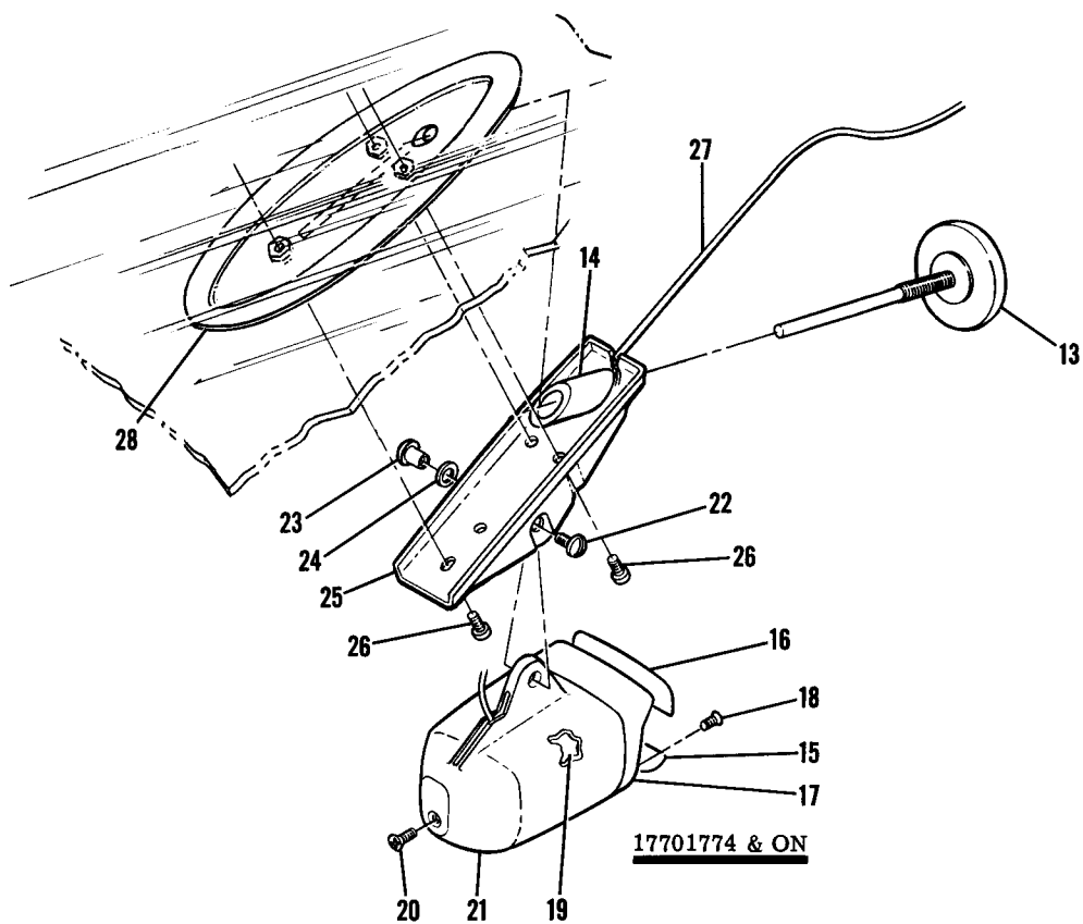
Figure 47A. Compass &amp; Outside Air Temperature Installation
