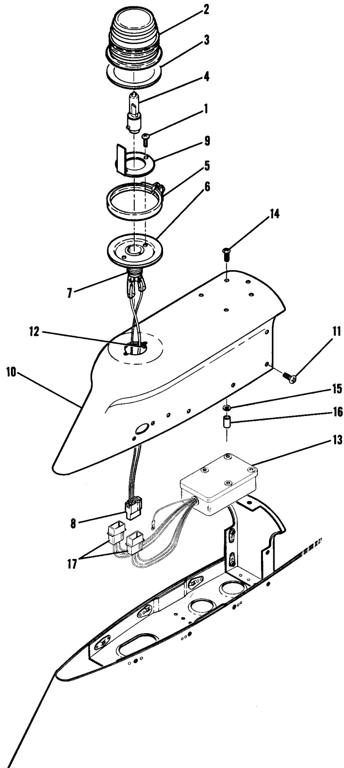
Figure 80. Flashing Beacon Installation
