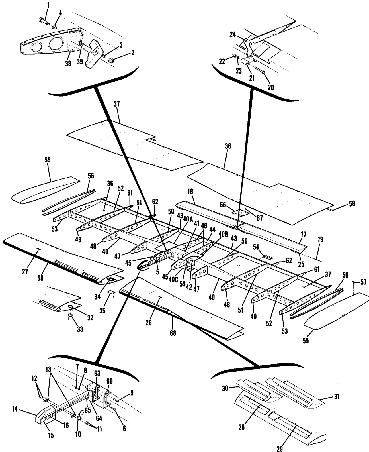
Figure 11. Stabilator Installation
