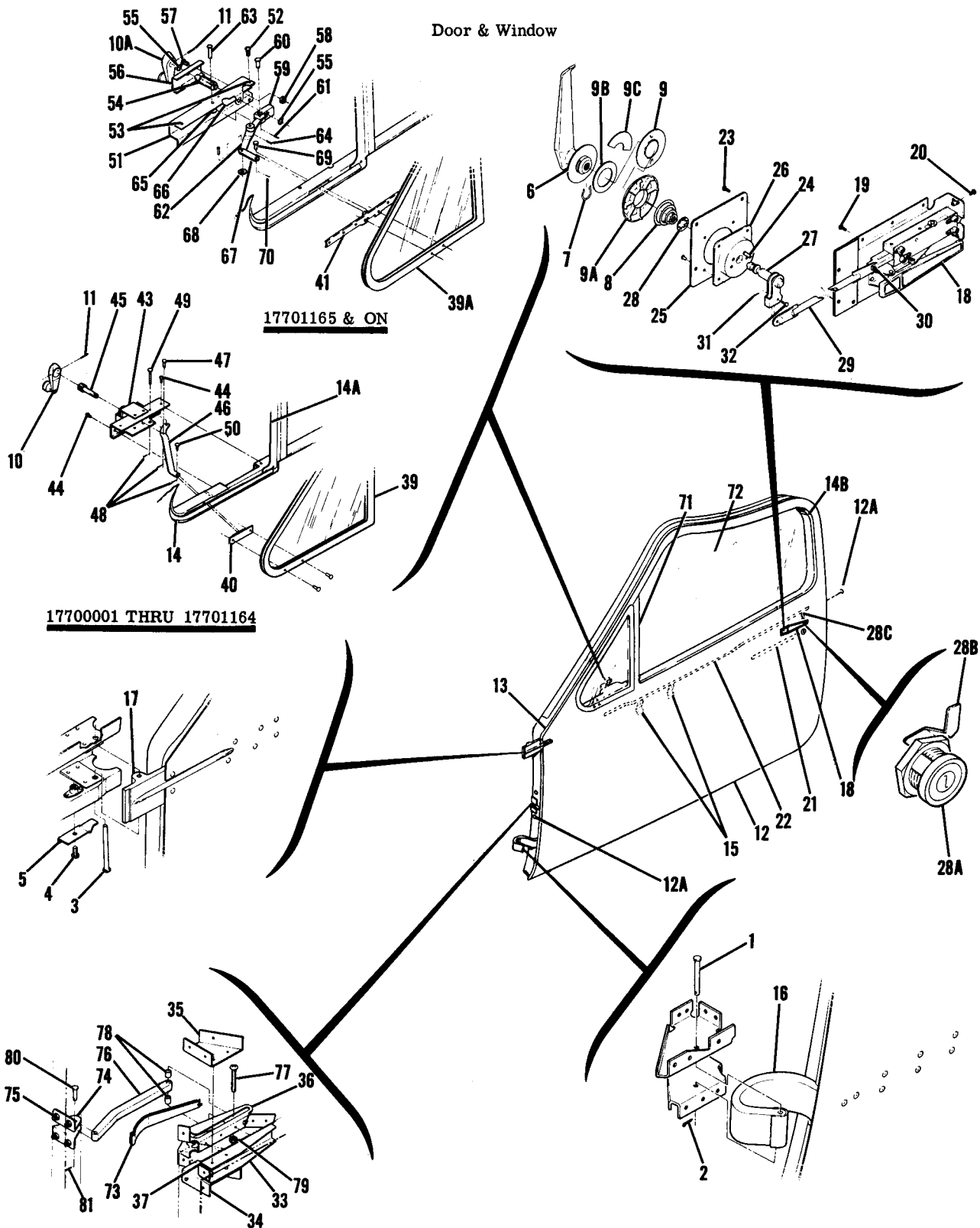
Figure 35. Cabin Door Assembly
