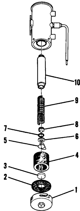
Figure 72. Auxiliary Fuel Pump Assembly
