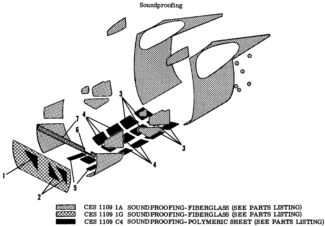
Figure 40A. Cabin Soundproofing Installation
