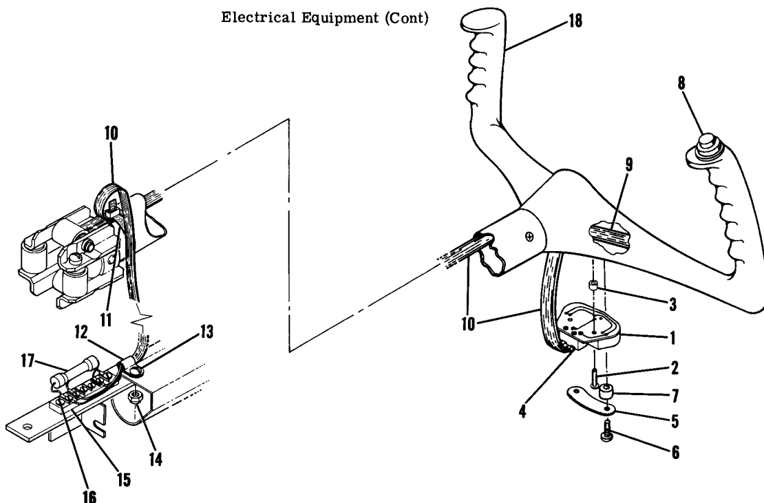
Figure 82. Control Wheel Map Light &amp; Mike Switch Installation
