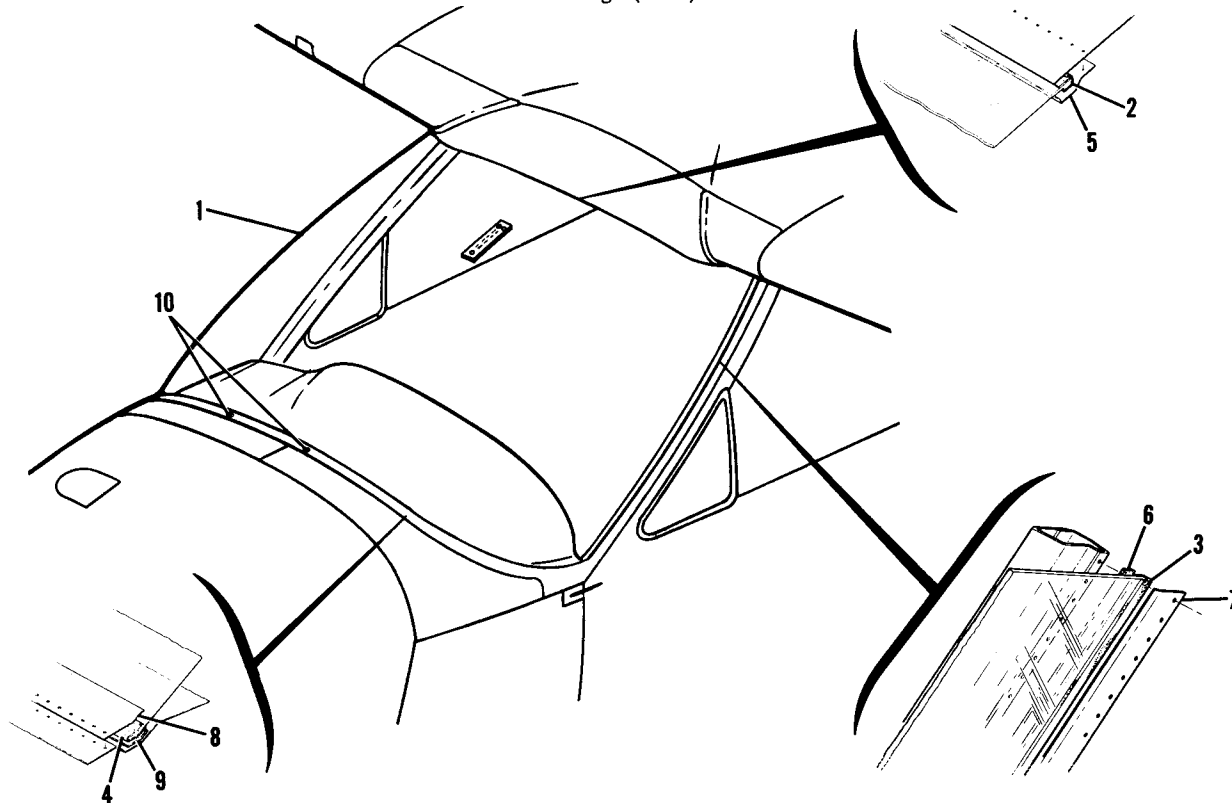
Figure 21. Windshield Installation
