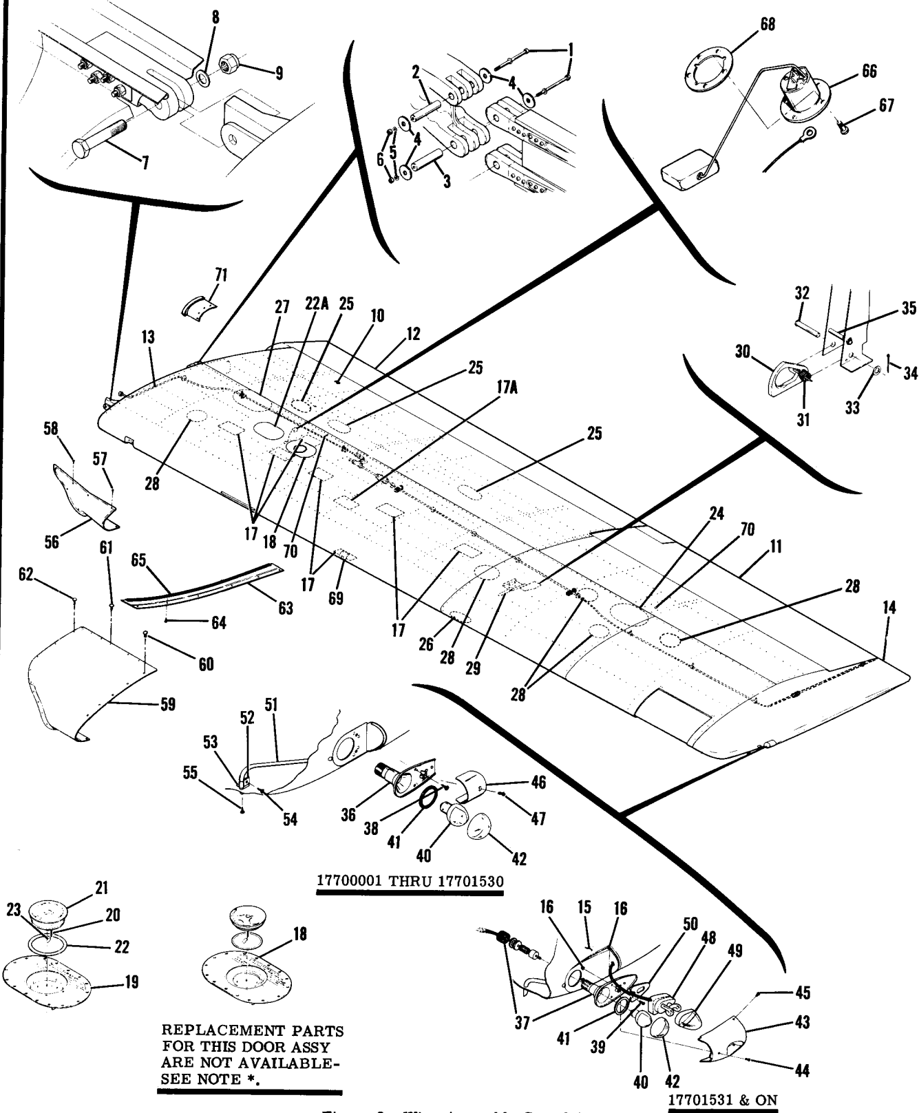
Figure 3. Wing Assembly Complete
