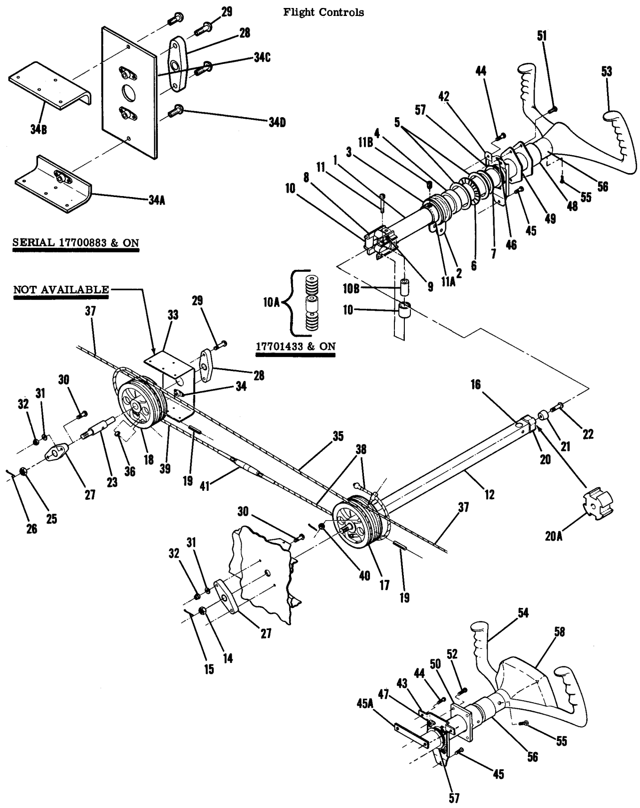
Figure 61. Control Column Installation
