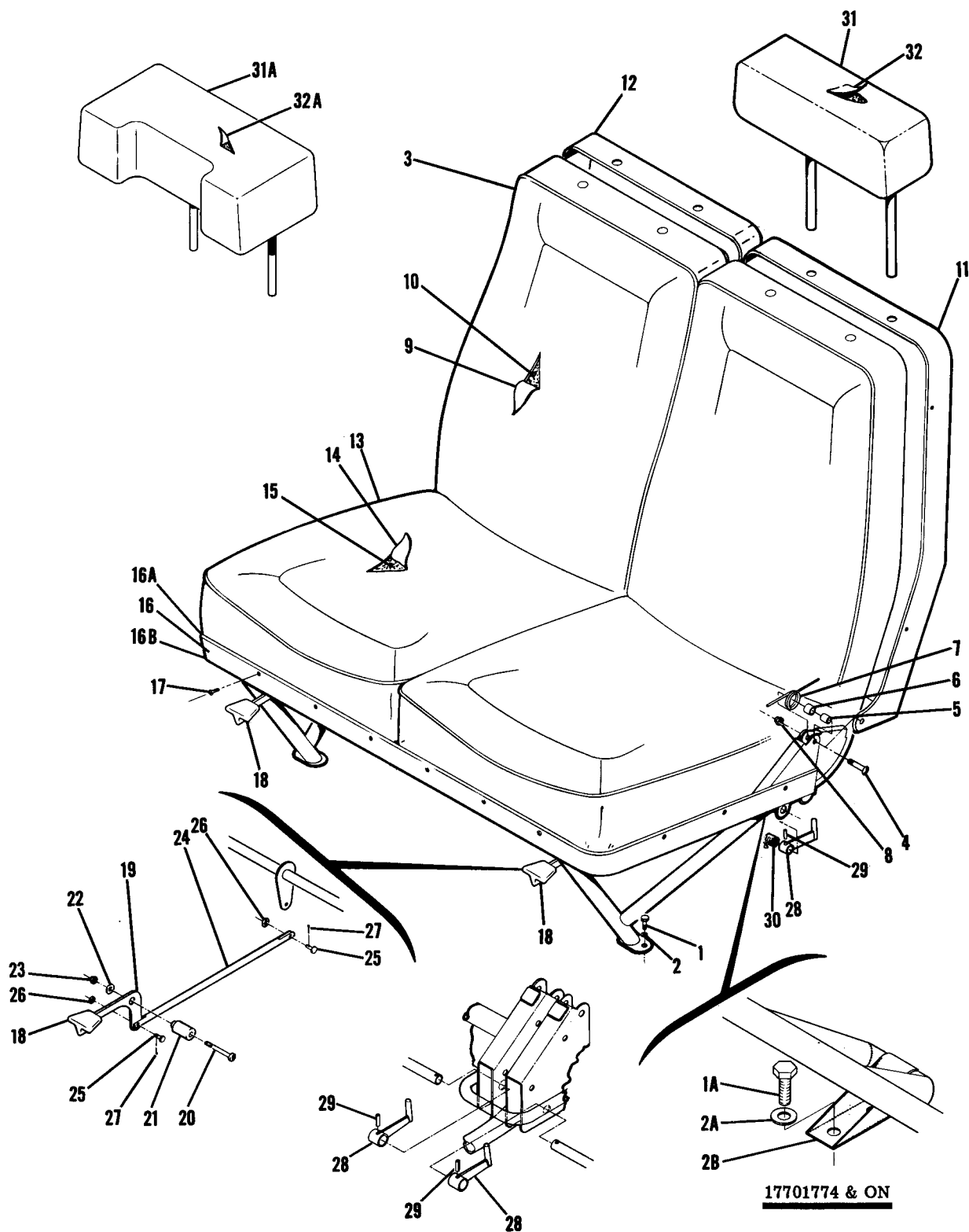
Figure 43A. Rear Seat Installation-Individually Reclining Back
